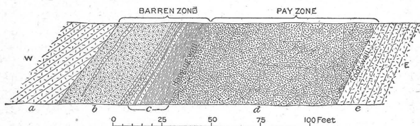
FIGURE 4.—Section across the cerusite belt near Ilse, Custer County, Colo., at the open cut of the Terrible mine. a , Gneissoid granite; b , disintegrated diorite; c , clay gouge with fragments of granite material; d , crushed, altered, and iron-stained granite with calcite and pockets of cerusite; e , granite.
