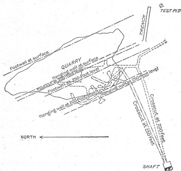
FIGURE 5.—Plan of the Terrible mine, near Ilse, Custer County, Colo.
