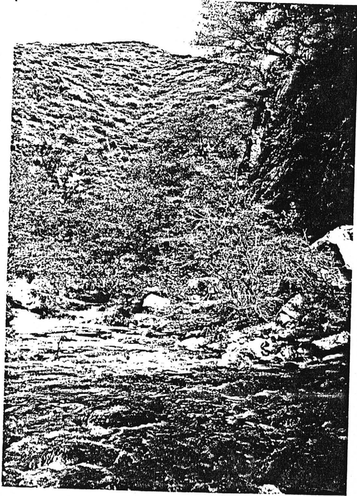
Figures 14 and 15: Gazelle Vein. Vein outcrops on both W and E sides of Humbug Creek and presumably underlies the creek (as seen in flood, above) for a total thickness of about 40 feet. A new exposure (site of sample G-1) blasted by the Karry family reveals fresh sphalerite, galena, pyrite, and chalcopyrite in white quartz. Samples there average 0.08 oz/t Au, 1.4 oz/t Ag, and visually estimated 5% Zn, 1% Pb, 0.5% Cu.
