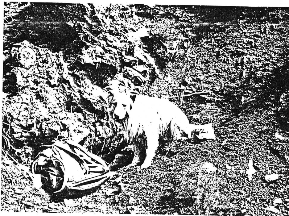
Figure 13: Outcrop of Gazelle vein just above field of view in Figure 12. Note bold outcrop of nearly barren quartz over dog's head versus the poorly exposed iron-stained, gossanous, more precious-metal rich zone where the rock hammer lies. Quartz assays 0.006 oz/t Au, 0.3 oz/t Ag, Gossan (G-21) assays 0.04 oz/t Au, 3.7 oz/t Ag.
