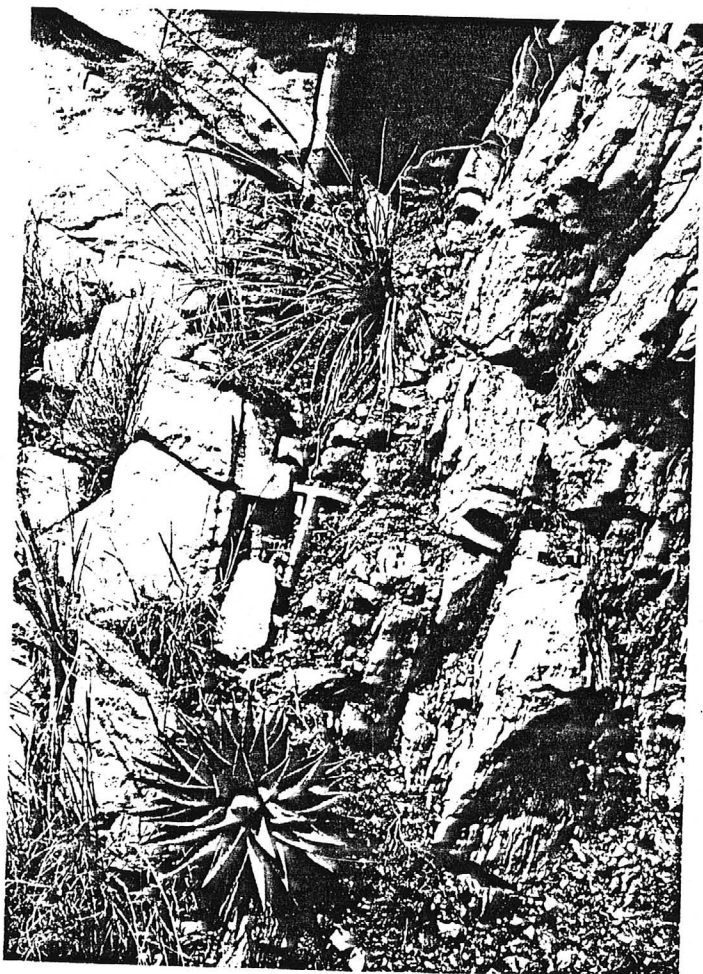
Figure 10 and 11: Gabbro dike showing conformable contact with Precambrian wall rock and close-up of fresh gabbro surface showing calcic plagioclase phenocrysts in a finer grained pyroxene-hornblende-biotite groundmass. Samples of the gabbro and wall rock all assayed 0.001 oz/t Au or less, indicating the dikes are not critical to the mineralization.
