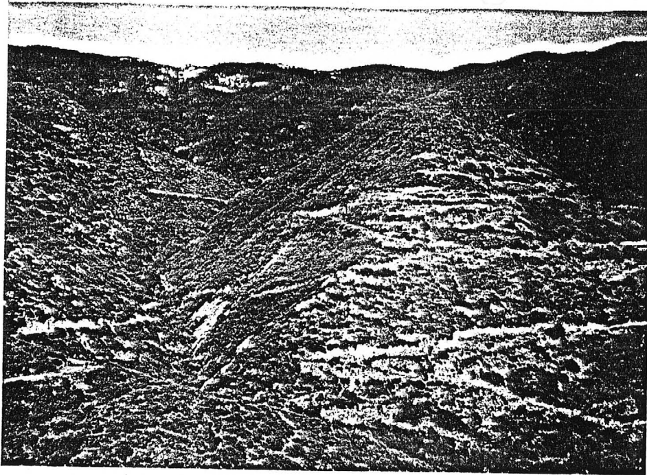
Figure 8: View E, up Humbug Creek to the OroBelle mine area near the pegmatitic batholith on the skyline, with zig-zag dozer cuts of the Antelope area closer right.
