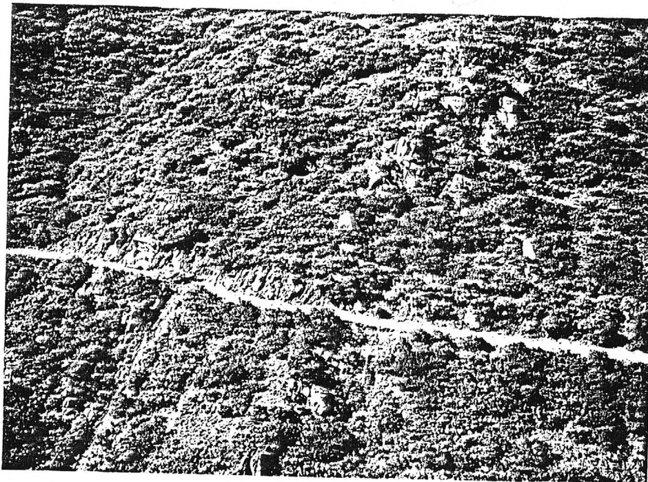
Figure 12: View N from the Antelope adit to the south slope of Wasson Peak revealing the steep westerly dip of the Precambrian bedded rocks, the more prominent exposures of two Cretaceous (?) gabbro dikes, and the trace of the Gazelle vein (swale in upper left).
