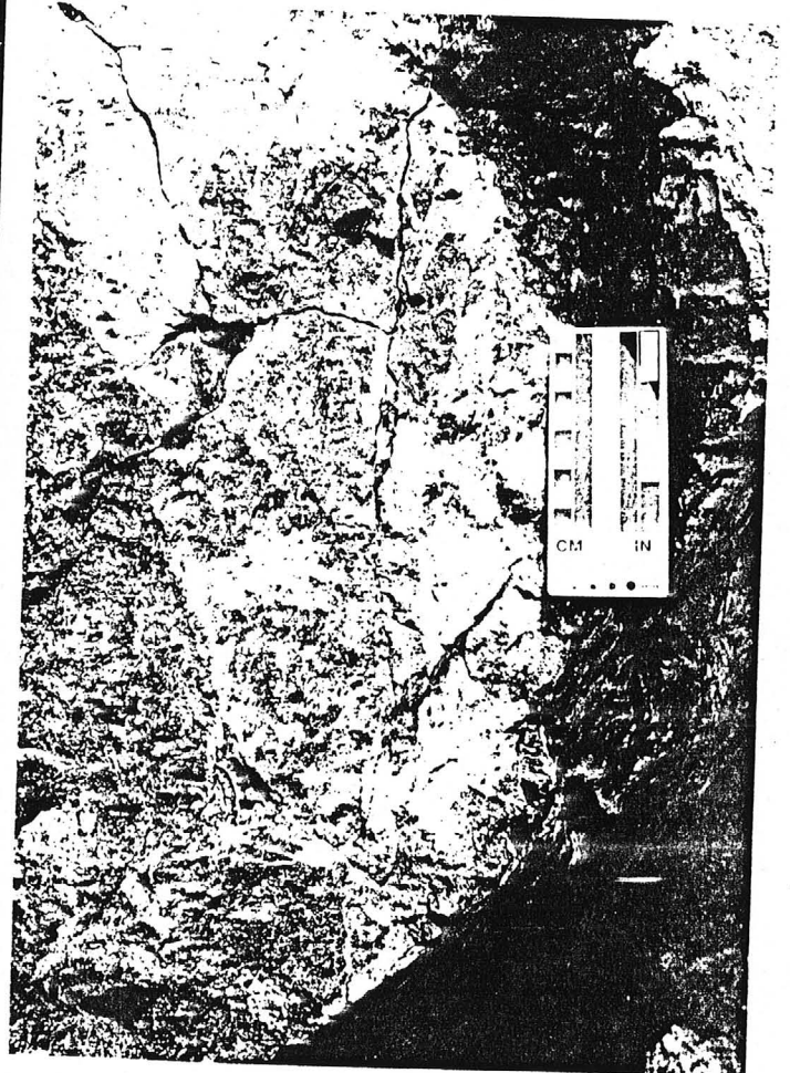
Figures 14 and 15: Gazelle Vein. Vein outcrops on both W and E sides of Humbug Creek and presumably underlies the creek (as seen in flood, above) for a total thickness of about 40 feet. A new exposure (site of sample G-1) blasted by the Karry family reveals fresh sphalerite, galena, pyrite, and chalcopyrite in white quartz. Samples there average 0.08 oz/t Au, 1.4 oz/t Ag, and visually estimated 5% Zn, 1% Pb, 0.5% Cu.
