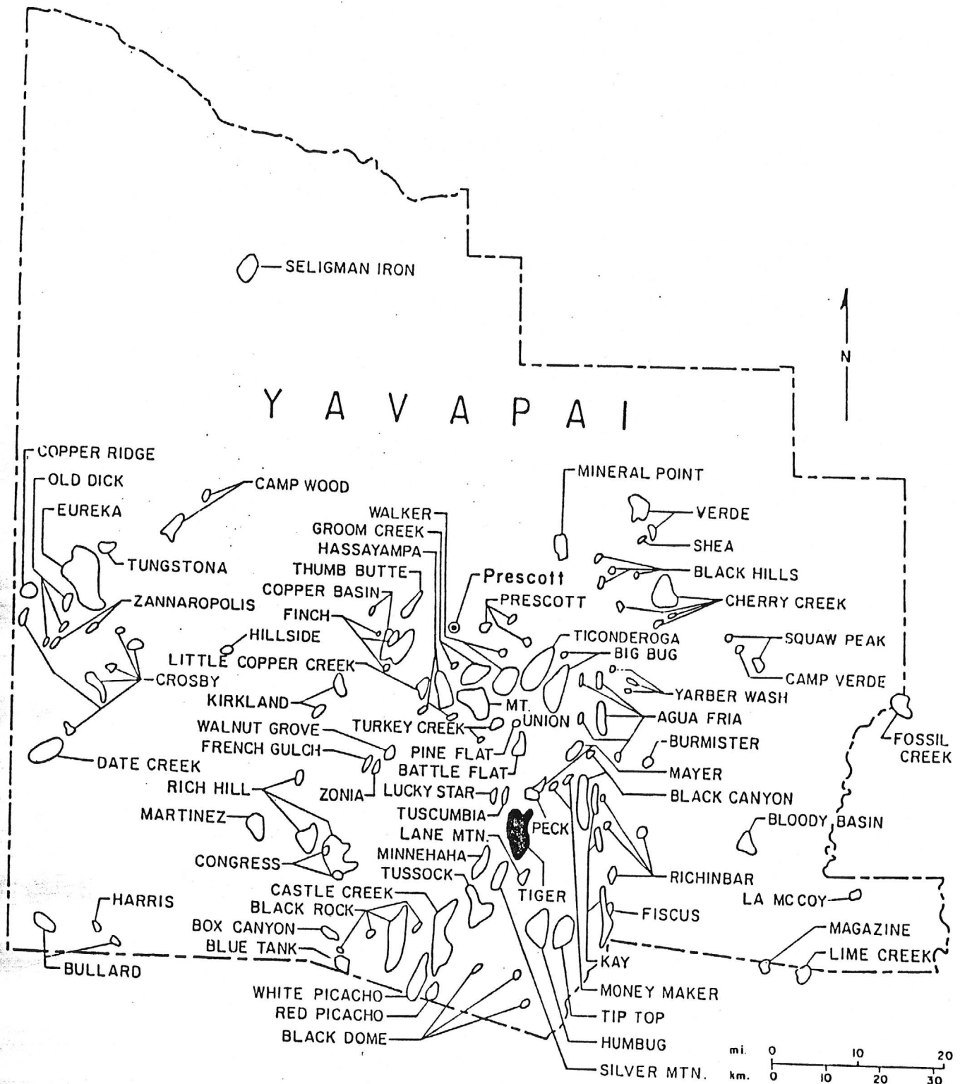
Mineral districts in YAVAPAI County, Arizona. Figure 16
