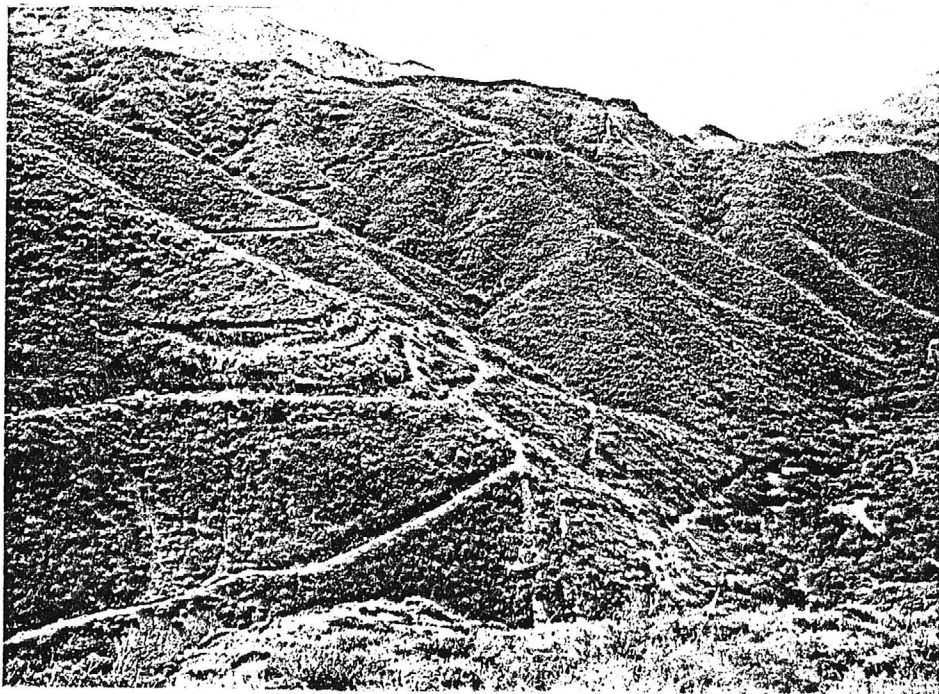
Figure 9: View S, looking down Humbug Creek along Gazelle Vein (in creek, lower right) to Karry's cabin with dozer cuts to Antelope adits (lower adit, lower left; upper adit, left center).
