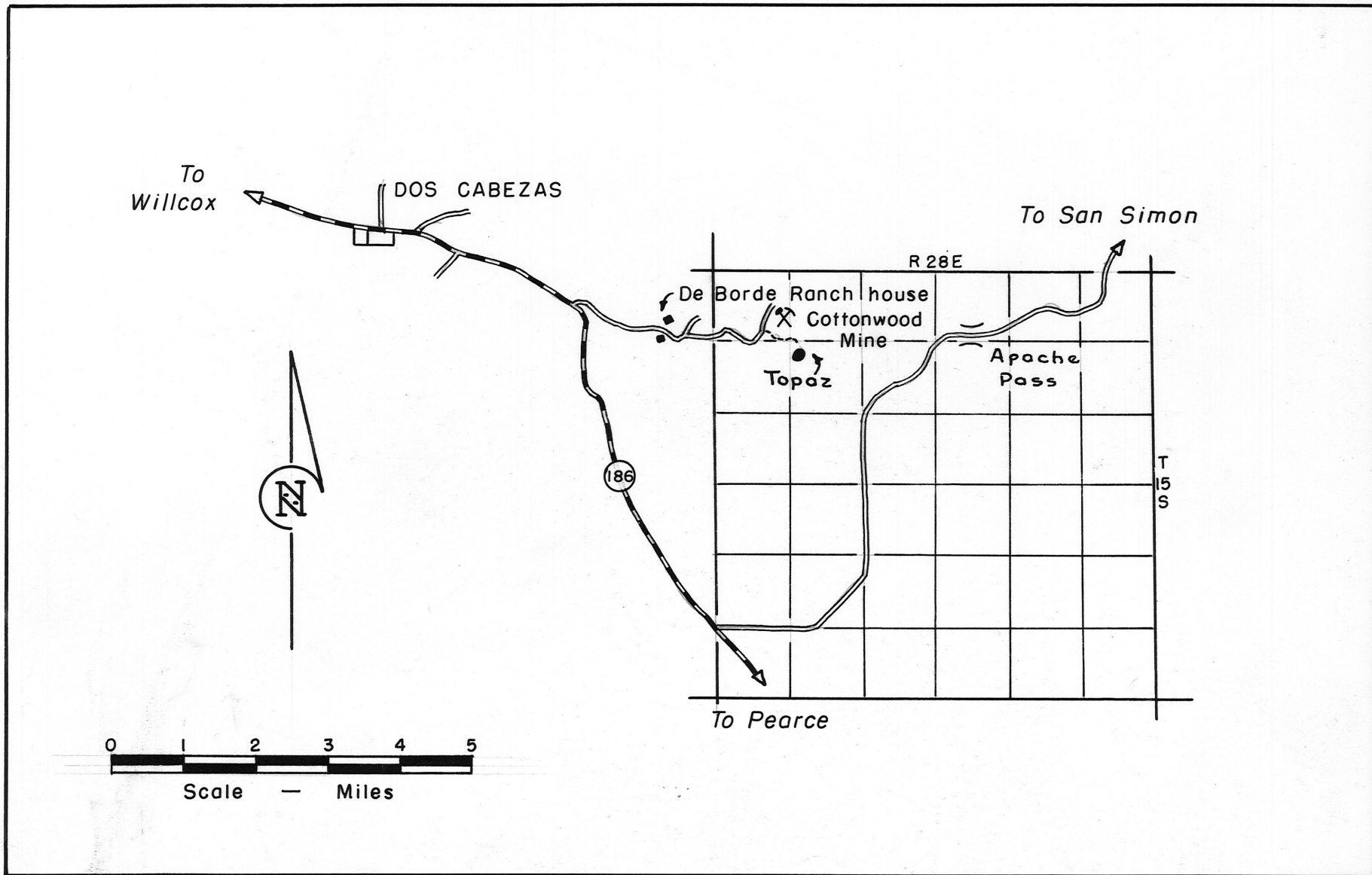
Fig. 1 Location map of Dos Cabezas Topaz deposit, Cochise County Arizona
