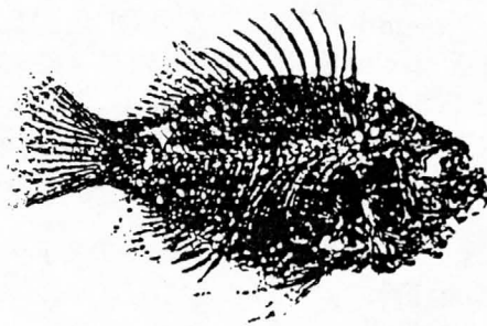
Eocene fish
