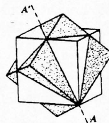
Isometric penetration twin. Fluorite crystal.
