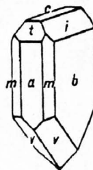
Orthorhombic system. Rhombic-pyramidal class. Hemimorphite crystal.
