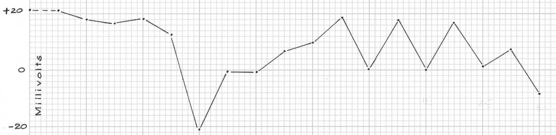
SELF POTENTIAL PROFILE
