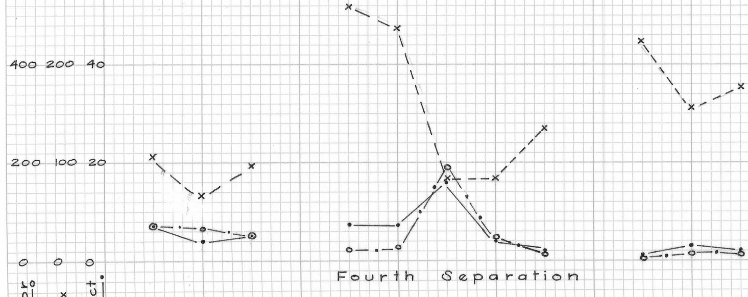
INDUCED POLARIZATION PROFILES
