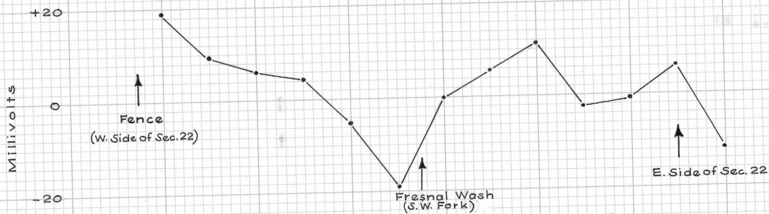
SELF POTENTIAL PROFILE
