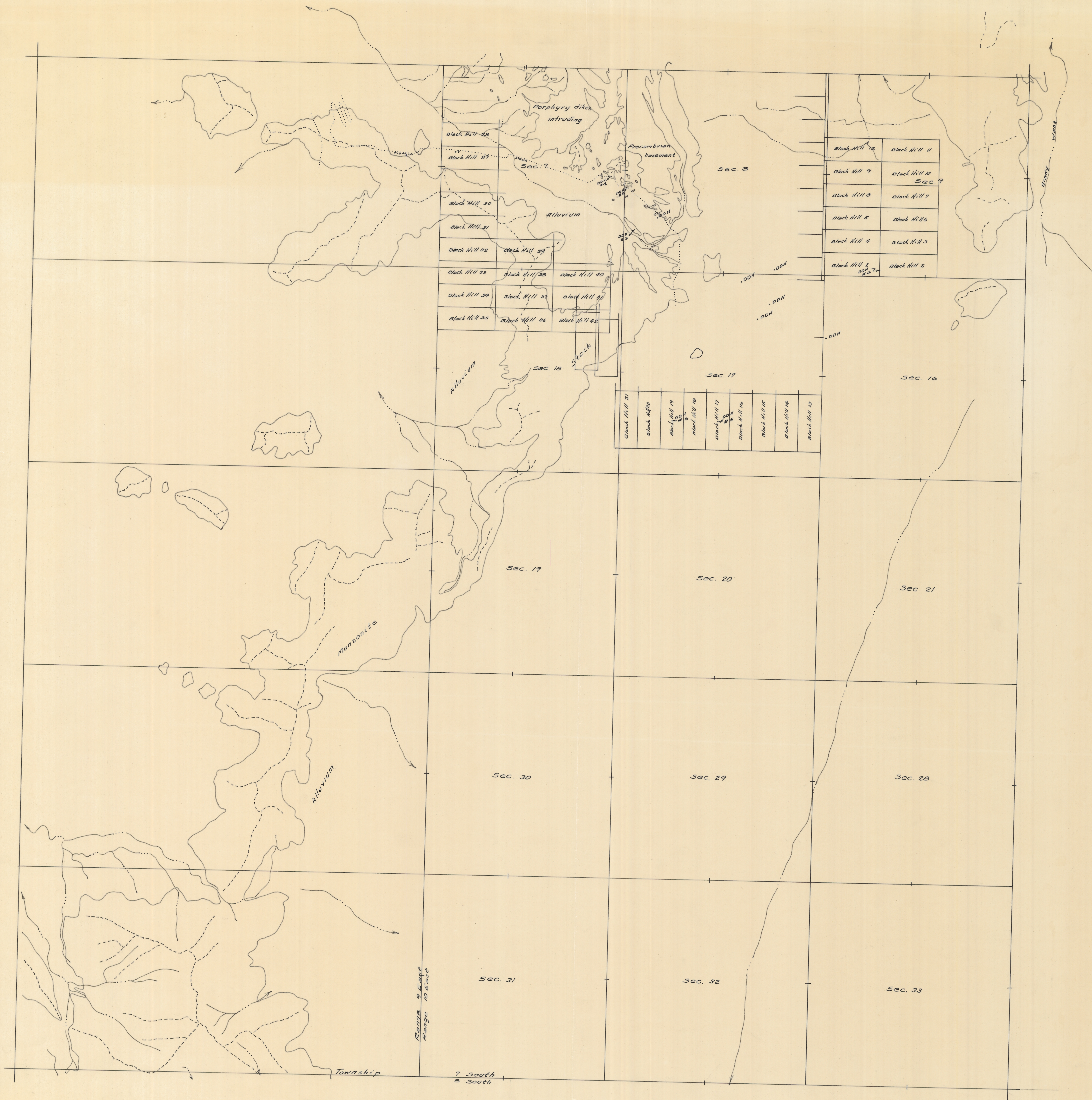
MAP OF PART OF THE NORTHERN PICACHO MOUNTAINS SHOWING BEDROCK OUTCROPS
