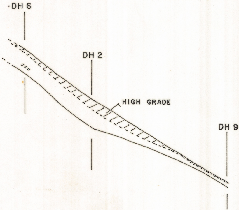
SECTION THRU DRILL HOLES 6, 2 & 9
