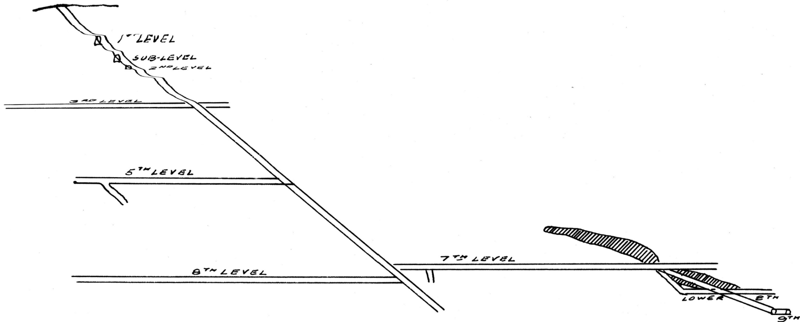
CROSS SECTION REPUBLIC MINE 50210 1" = 100'
