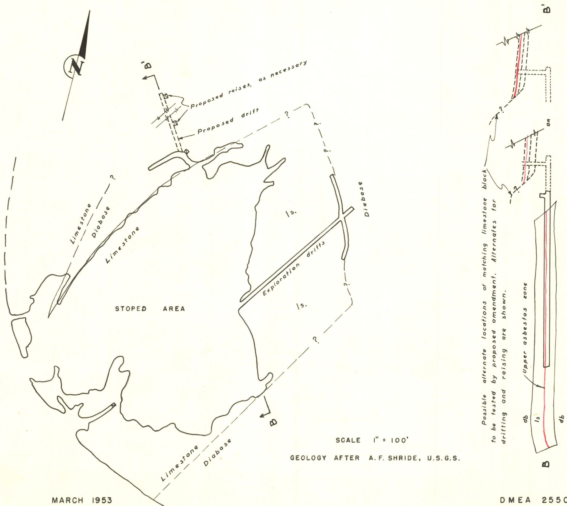
FIGURE A.- GENERALIZED GEOLOGICAL SKETCH, SHOWING PROPOSED AMENDED WORK
