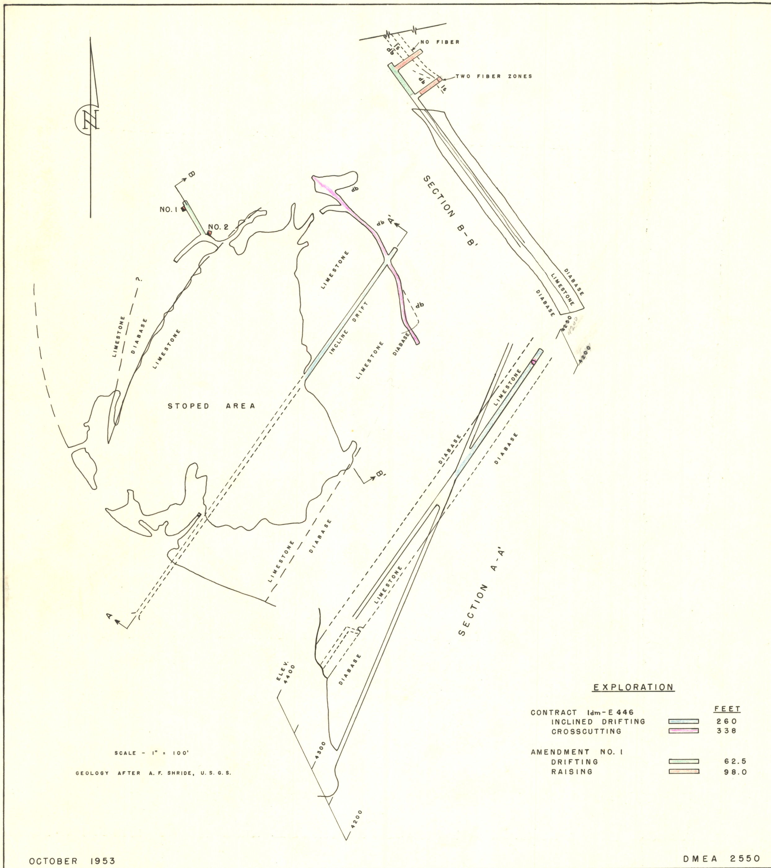
FIGURE 2. - GENERALIZED GEOLOGIC SKETCH SHOWING WORK PERFORMED UNDER CONTRACT Idm-E 446 BEAR CANYON ASBESTOS MINE GILA COUNTY, ARIZONA
