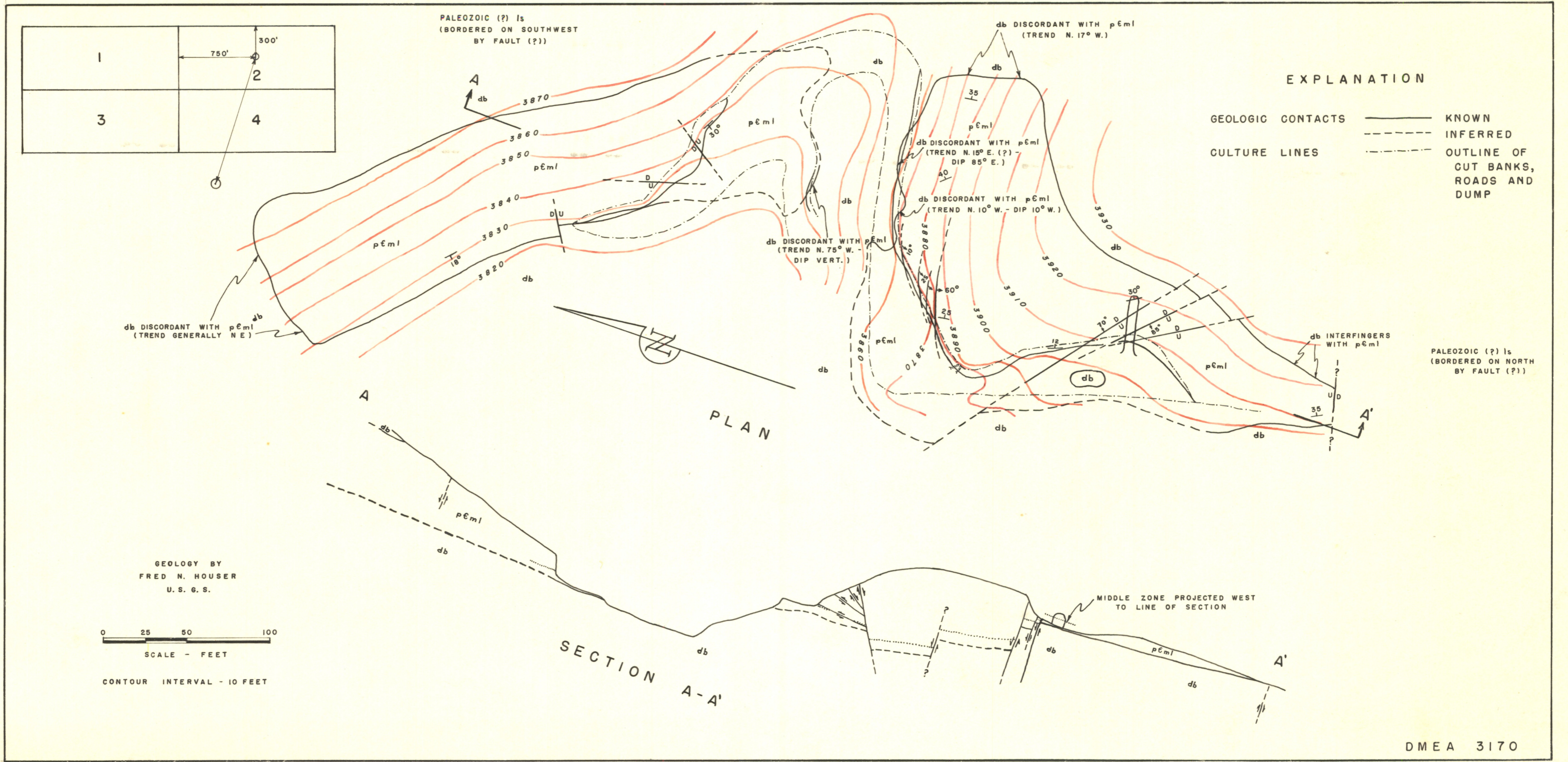
FIGURE 2. - PLAN AND SECTION OF THE MOUNTAIN OF MYSTERY CLAIM NO. 2 PINTO CREEK MINING DISTRICT PINAL COUNTY, ARIZONA
