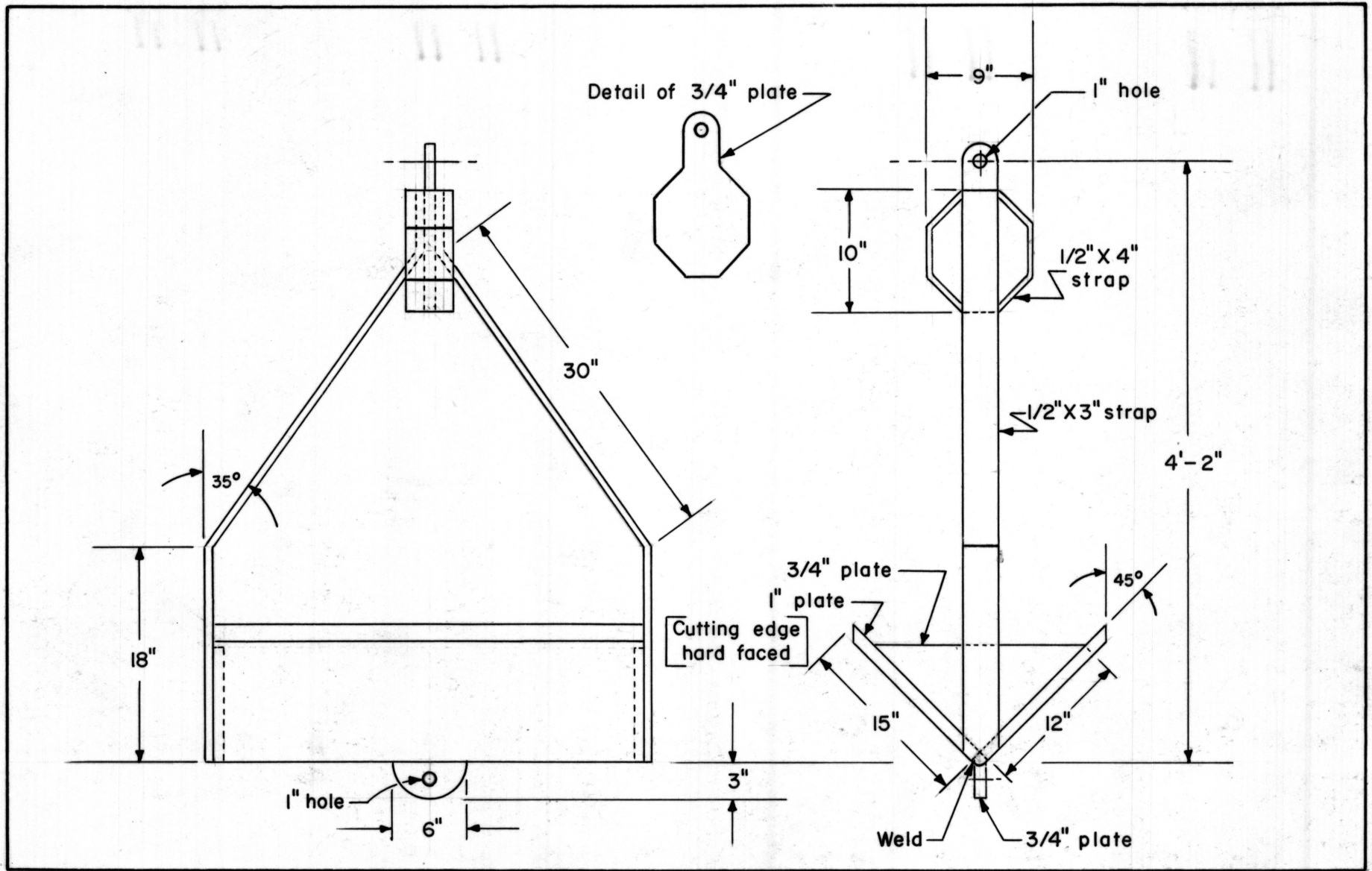
Figure 19. Detailed sketch of 36" scraper.
