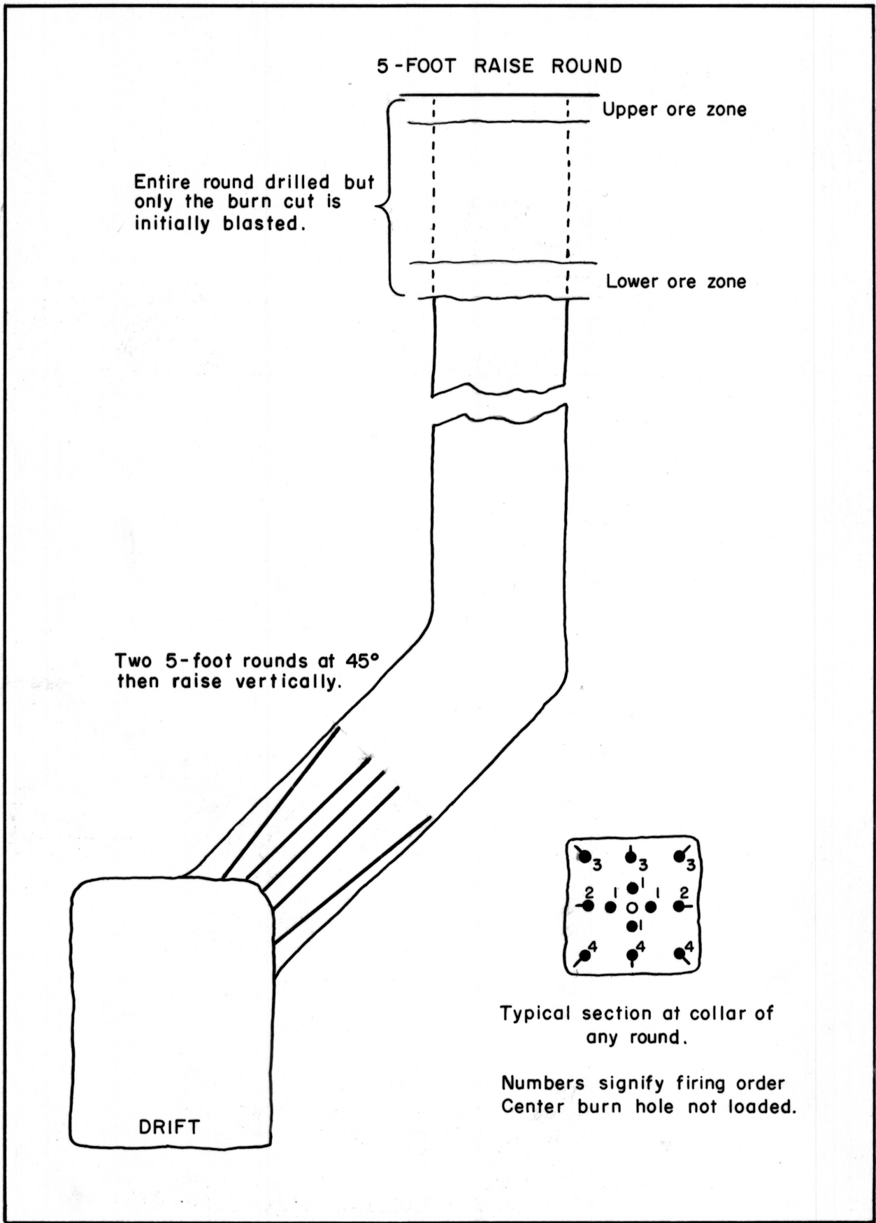
Figure 10. Development raise blasting round .
