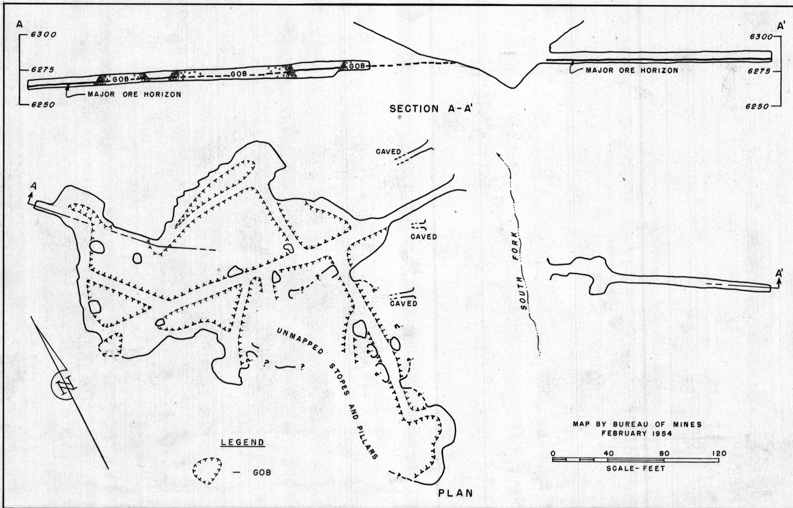
FIGURE 25. - PLAN AND SECTION OF REYNOLDS FALLS MINE
