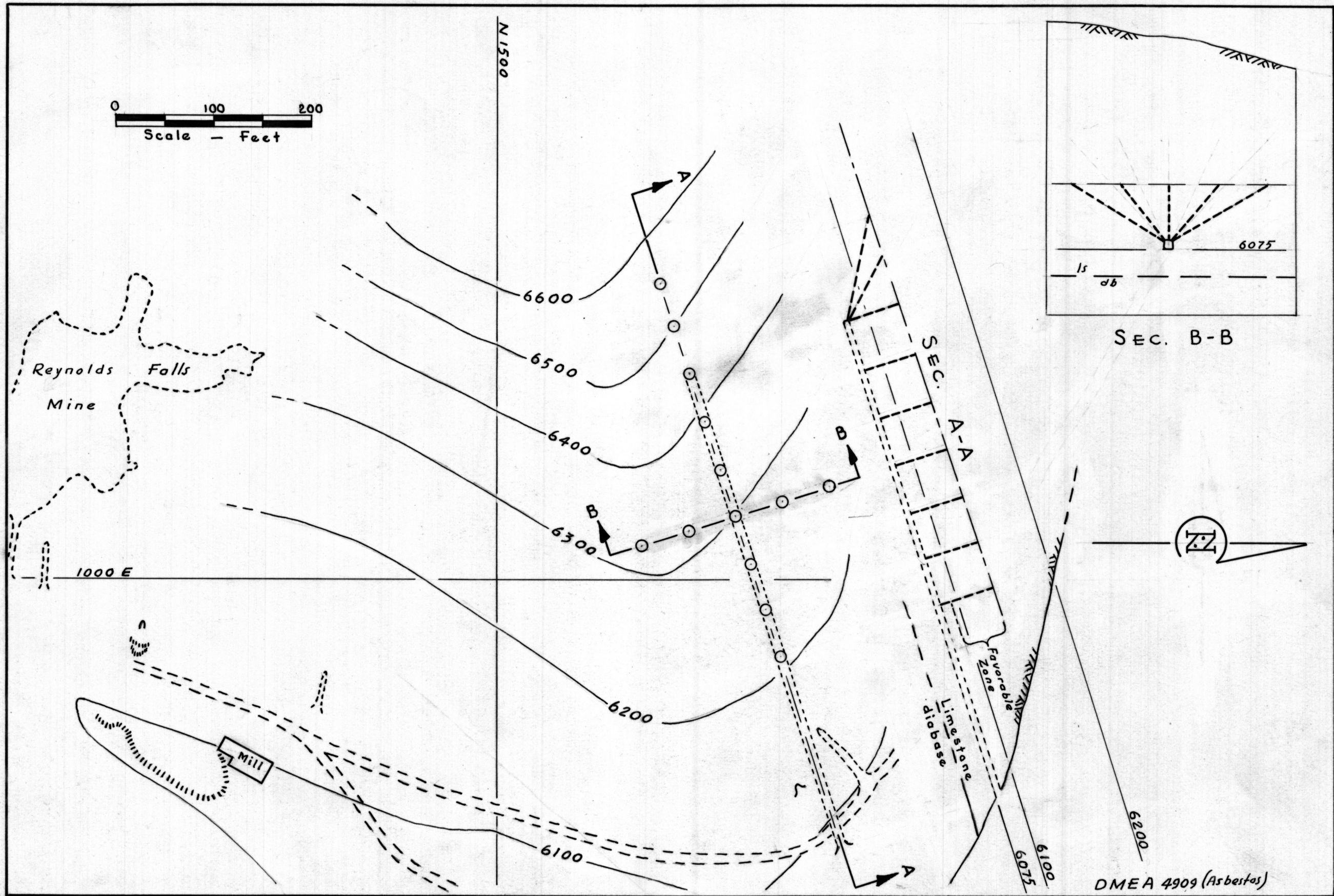
Fig. 5.- Proposed explorations, Reynolds Falls Asbestos Inc. Gila County Arizona
