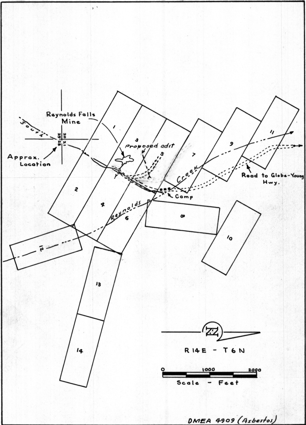
Fig. 2 Claim map, Falls Group, Reynolds Falls Asbestos Inc. Gila County, Arizona
