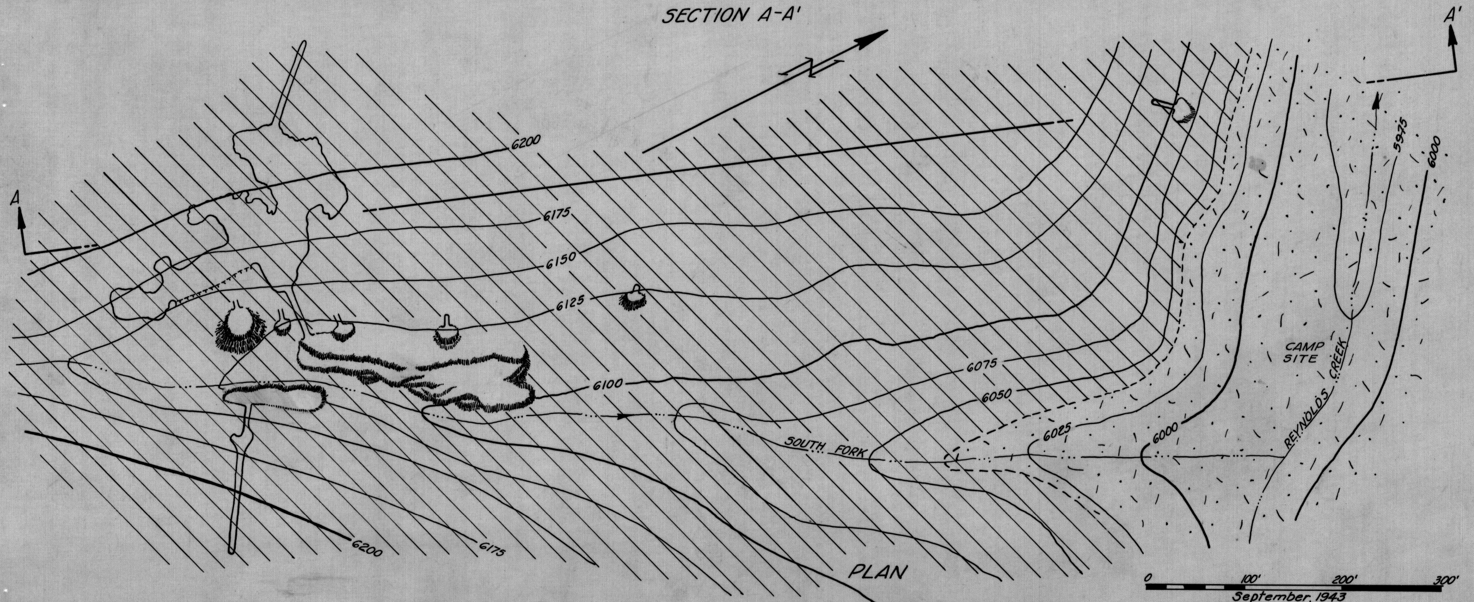
FIG. 25-PLAN & SECTION - REYNOLDS FALLS AREA - PROJECT NO. 2303
