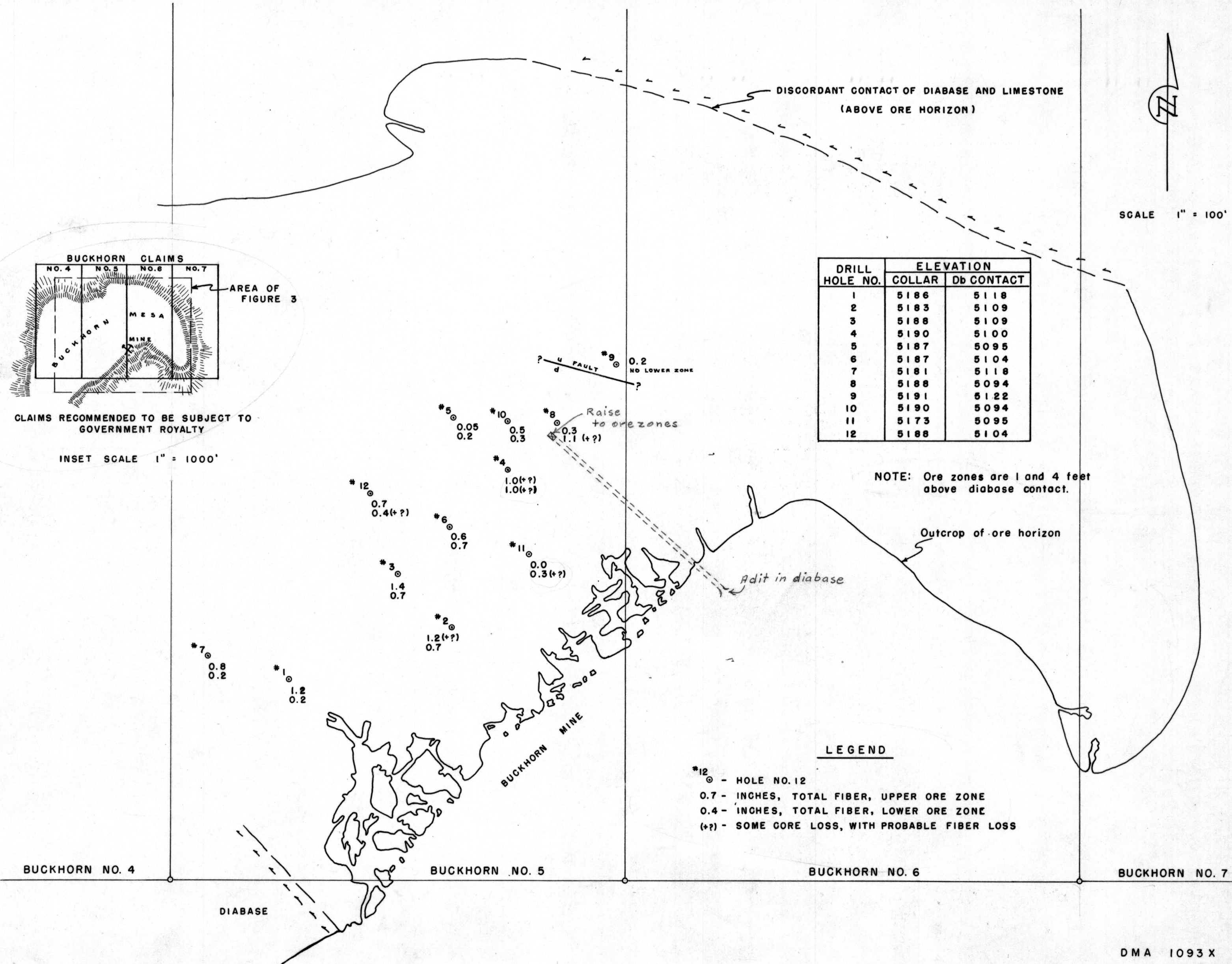
FIGURE 3. - PLAN OF BUCKHORN MESA SHOWING LOCATION OF DIAMOND DRILL HOLES AMERICAN ASBESTOS CEMENT CORPORATION, GILA COUNTY, ARIZONA
