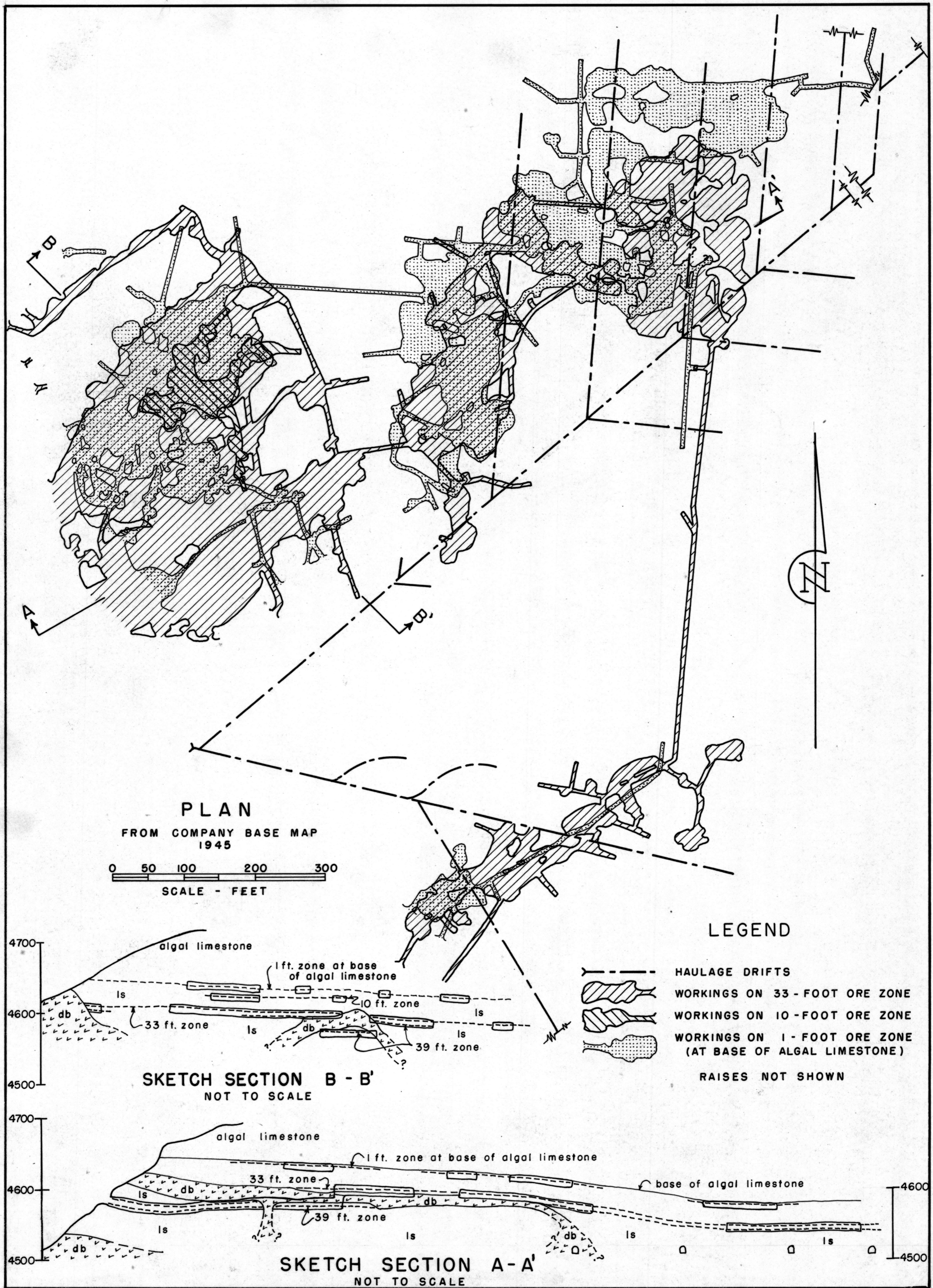
FIGURE 9. - PLAN AND SECTIONS - VICTORY MINE WESTERN CHEMICAL COMPANY (ASBESTOS DIVISION)
