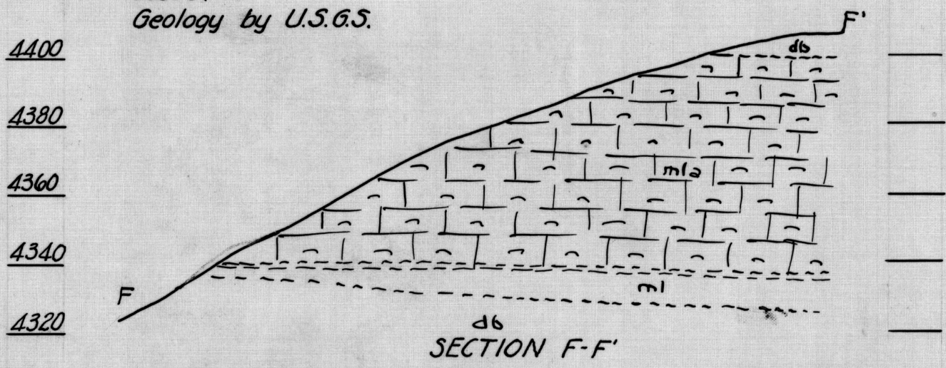
GEOLOGIC STRUCTURE SECTIONS-WHITETAIL CLAIMS Scale: 1"=40'
