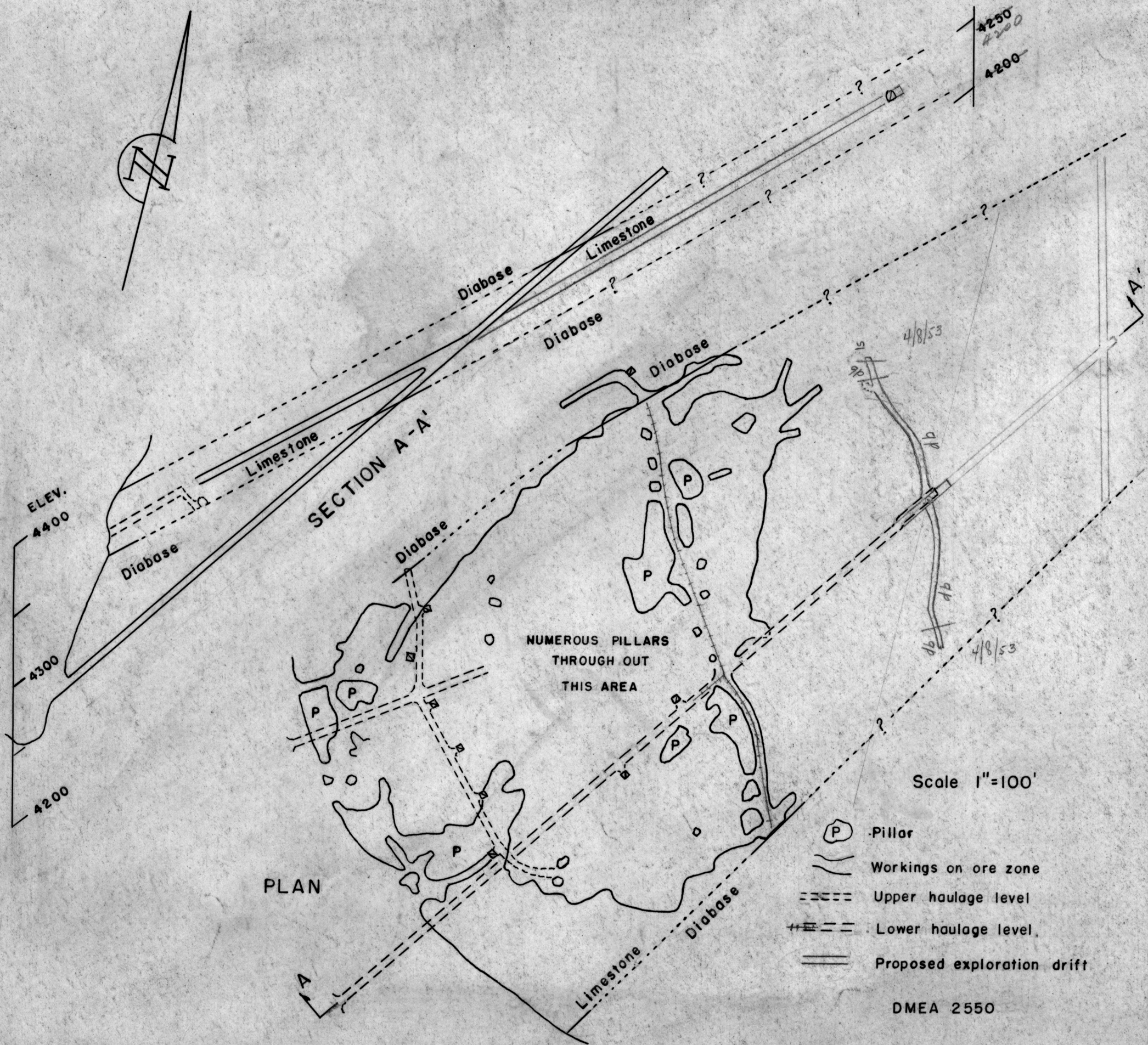
Figure 3— Plan and Section of Bear Canyon Mine, Showing Proposed Work
