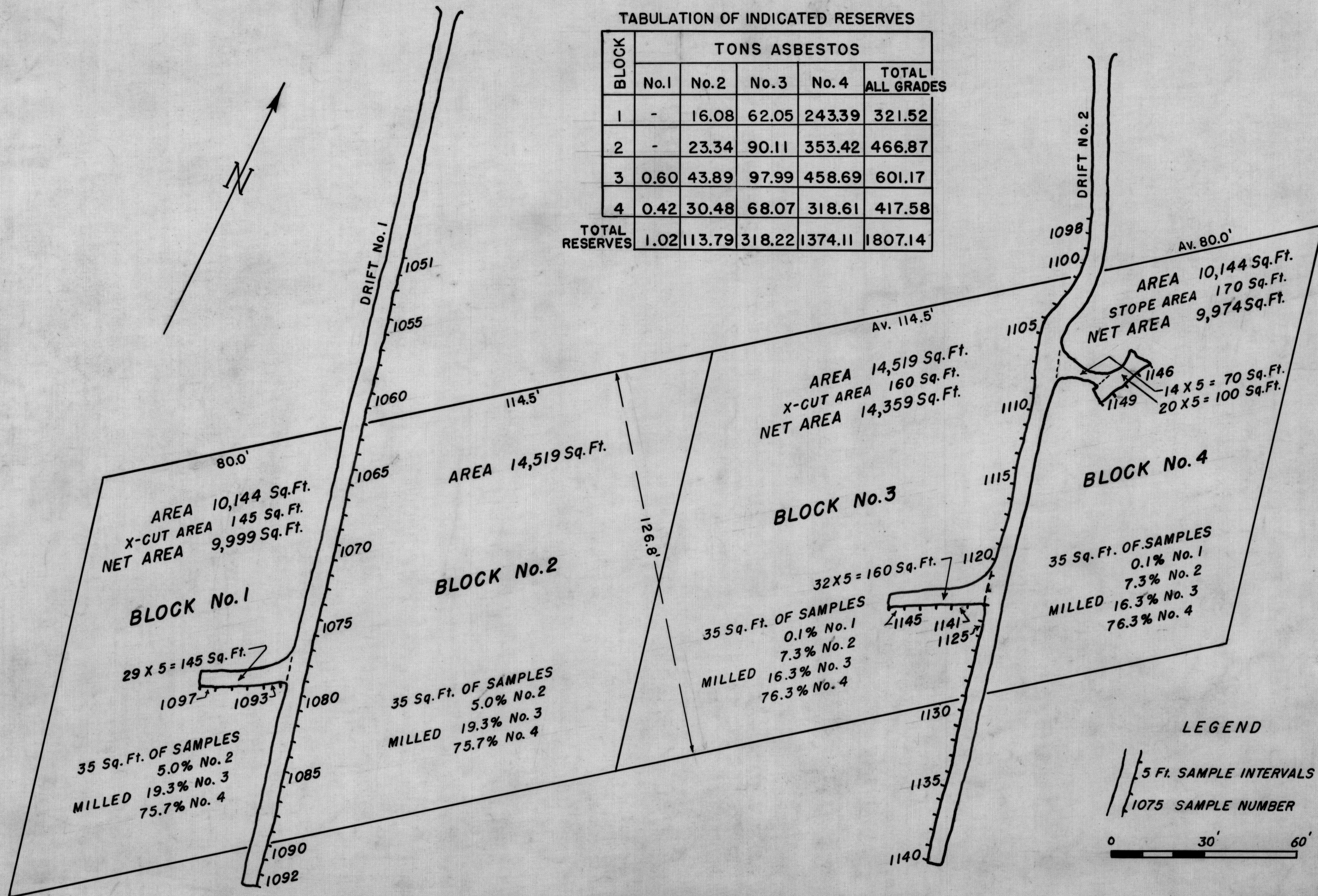
FIG.28- SAMPLE MAP & CALCULATIONS OF ORE RESERVES. PHILLIPS' GRANDVIEW No.4, PROJECT 2302
