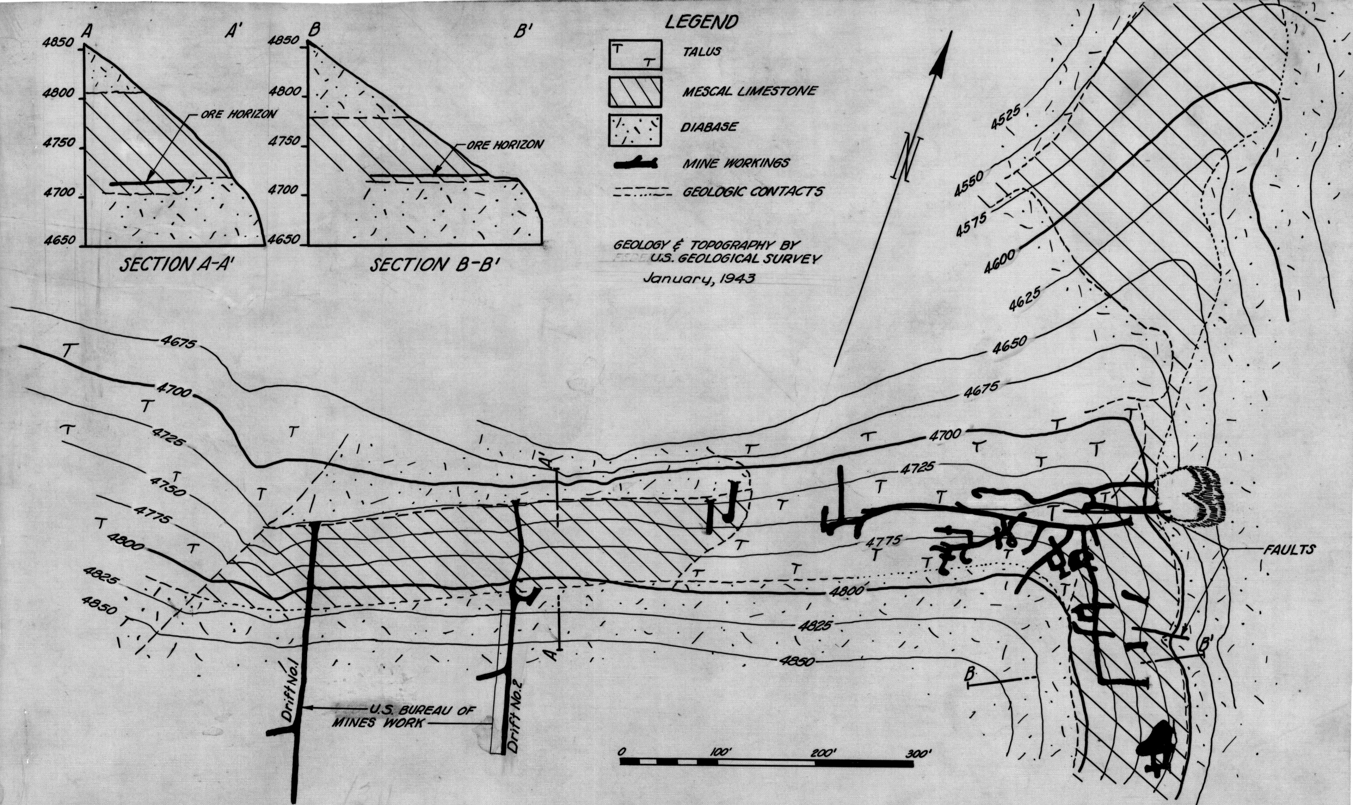
FIG. 16-PLAN & SECTIONS-GRANDVIEW CLAIMS NO. 4 & 5
