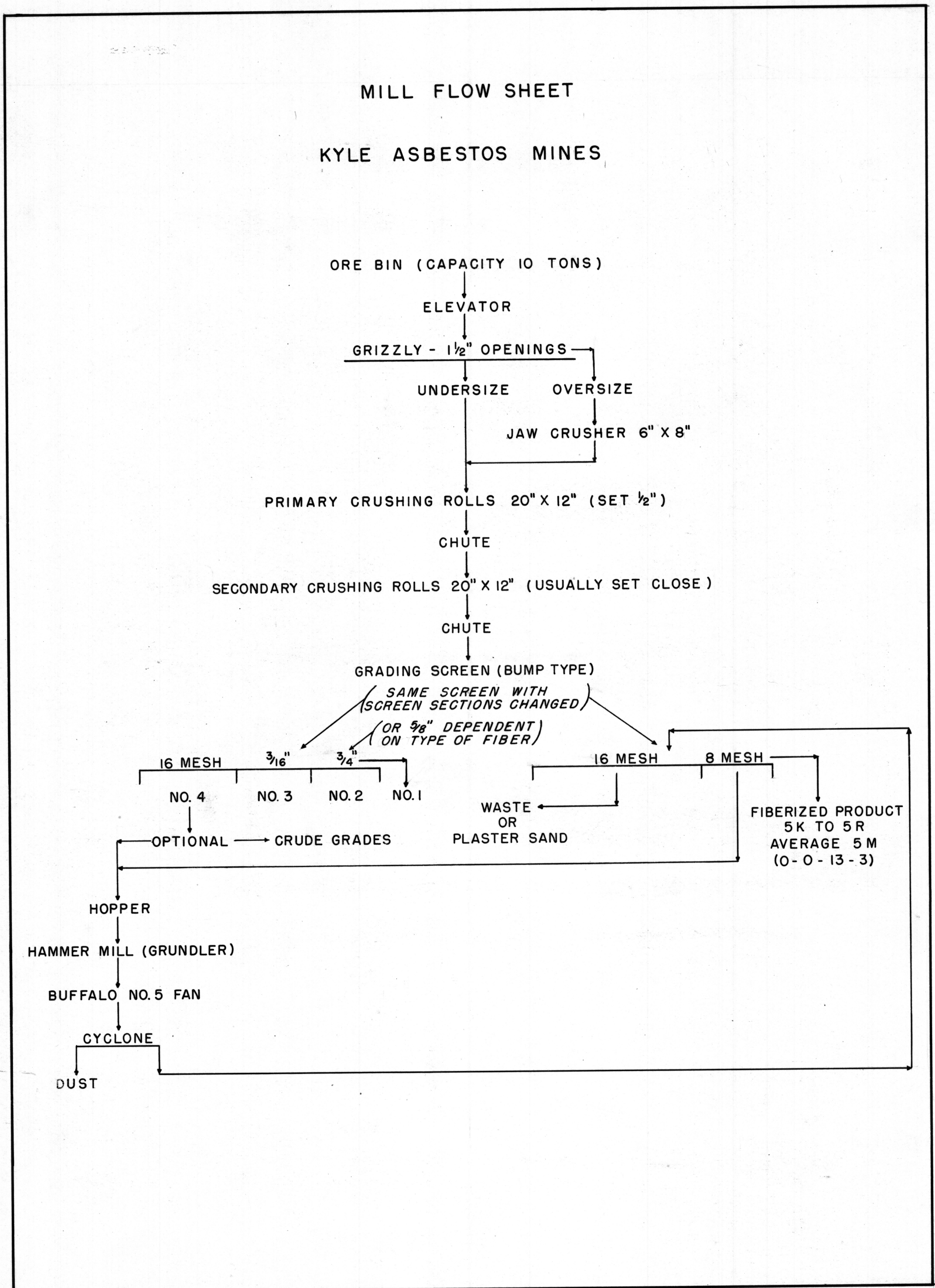
FIGURE 28. - MILL FLOW SHEET - KYLE ASBESTOS MINES OF ARIZONA
