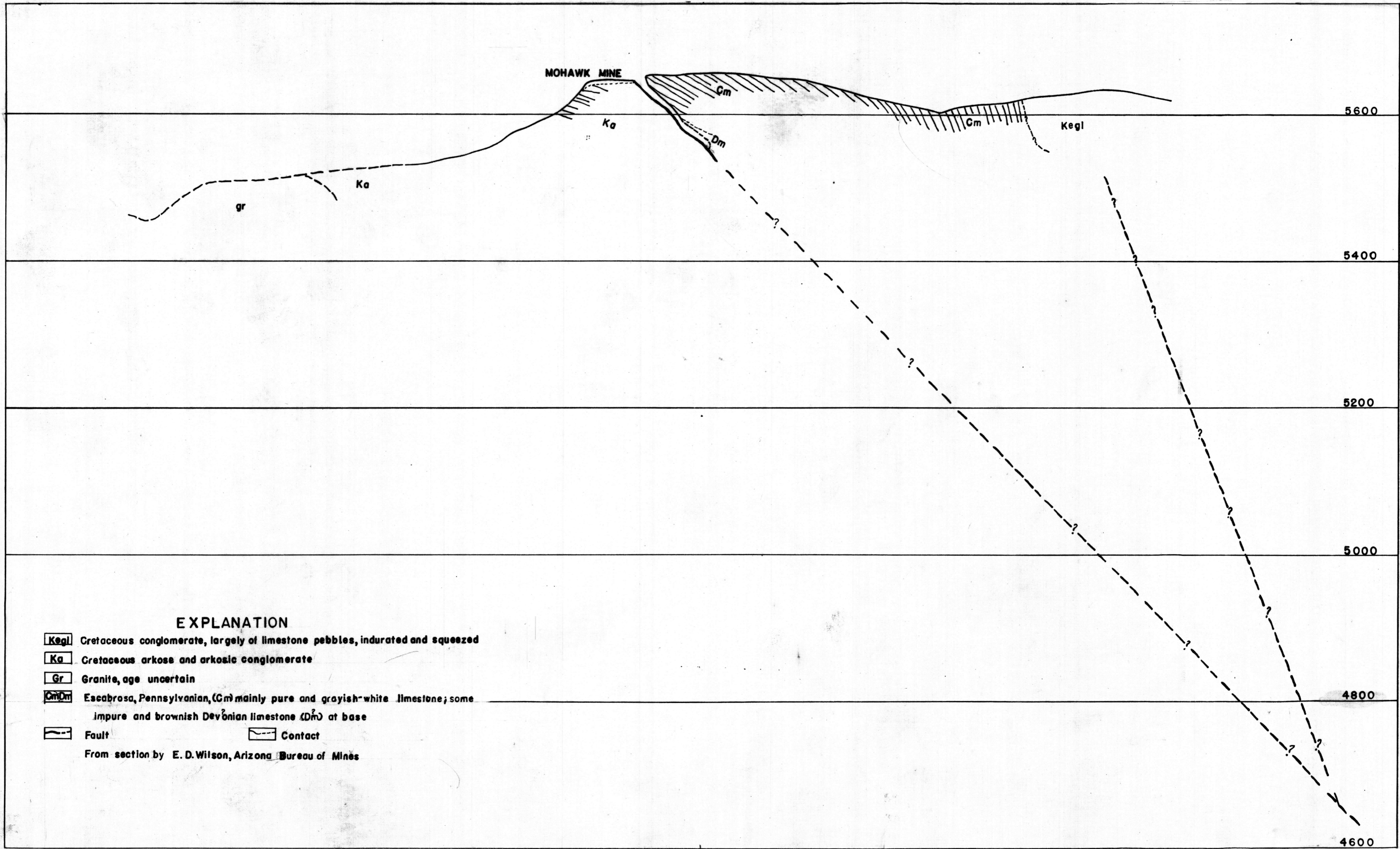
SECTION A-A', MOHAWK-SILVER ZINC DEPOSIT Scale 1"=100'
