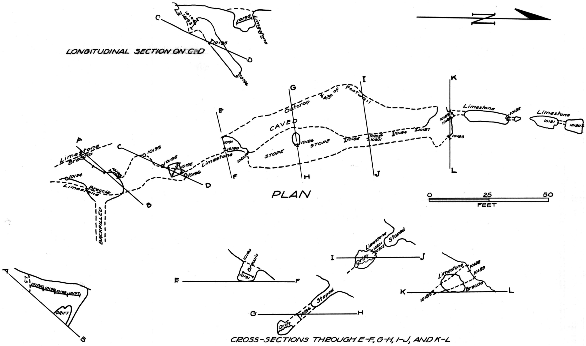
FIG. 6-SAMPLE PLAT SOUTH OUTCROPS & OLD WORKINGS, MOHAWK SILVER CLAIM-PROJ. 15-176
