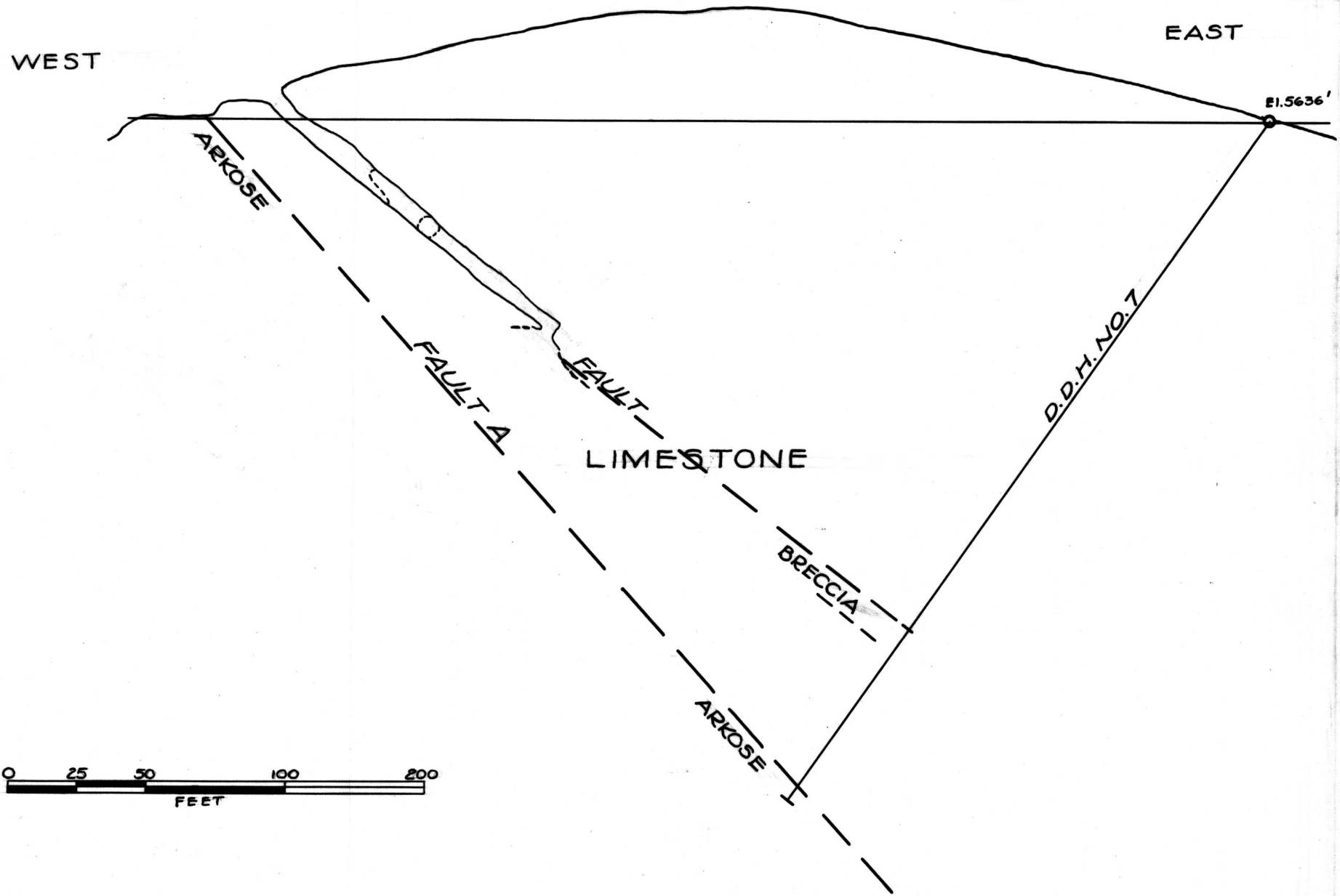
FIG. 5-SECTION THROUGH DRILL HOLE NO. 7, MOHAWK ZINC, PROJECT 15-176
