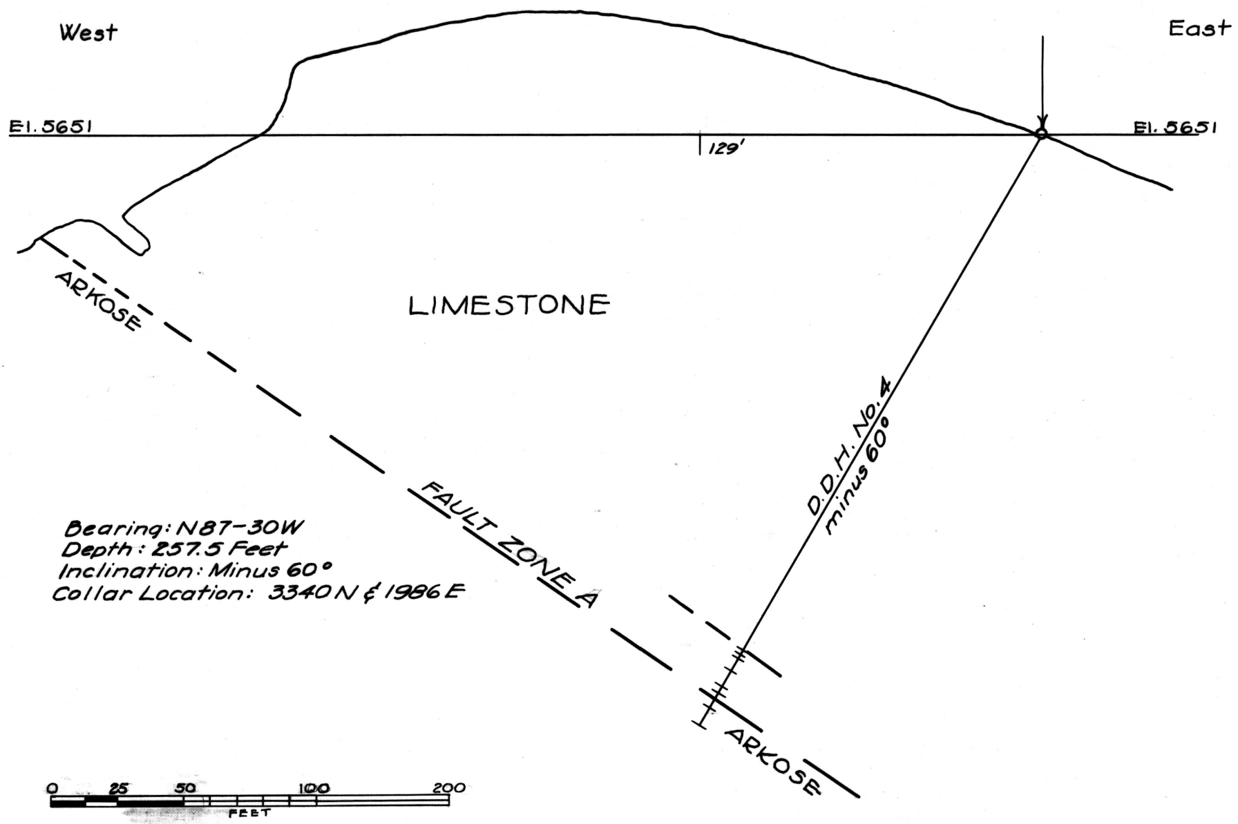
FIG. 4-SECTION THROUGH DRILL HOLE NO. 4, MOHAWK ZINC, PROJECT 15-176
