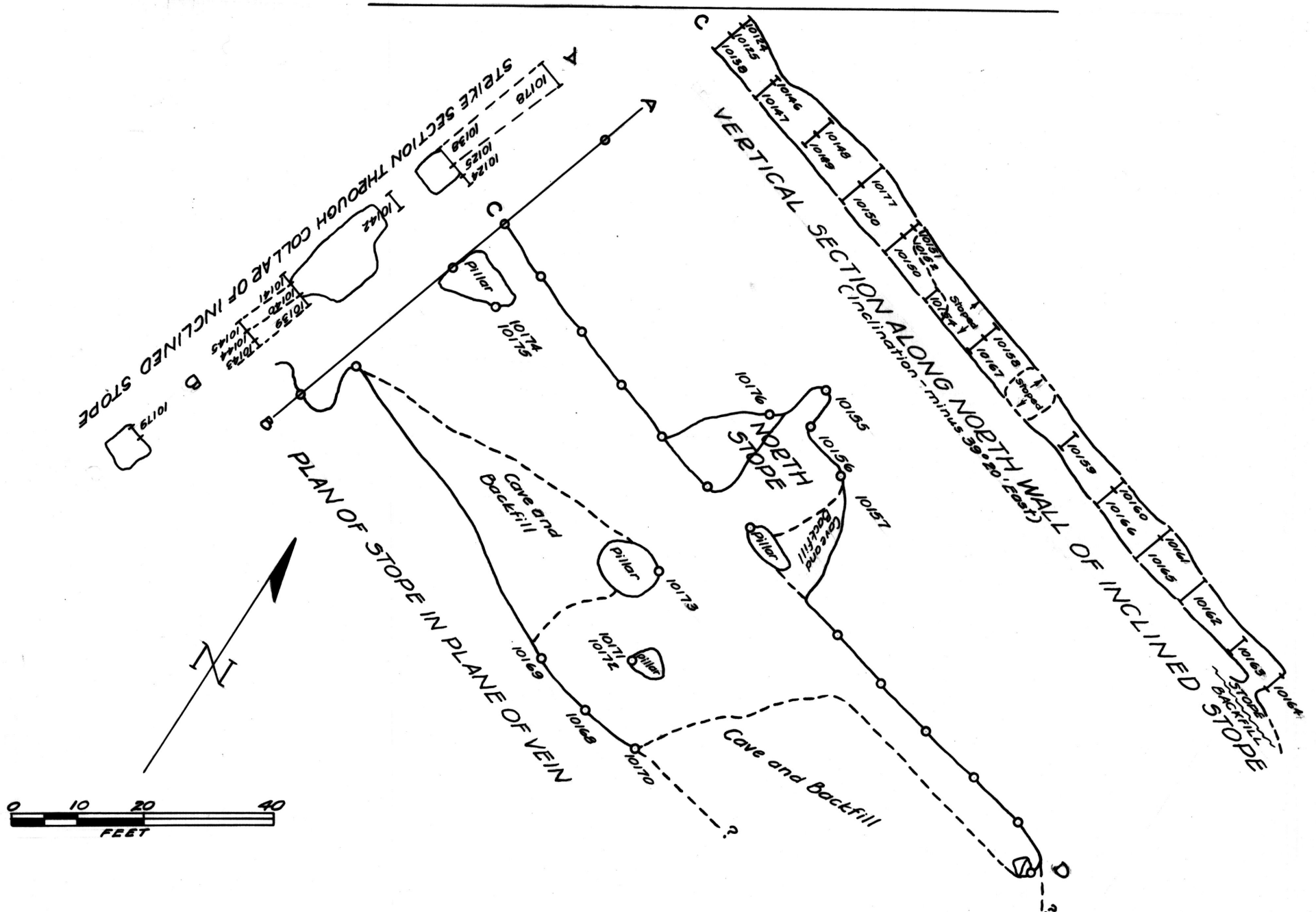
FIG. 7- STOPE NEAR NORTH END OF MOHAWK SILVER CLAIM, PROJ. 15-176
