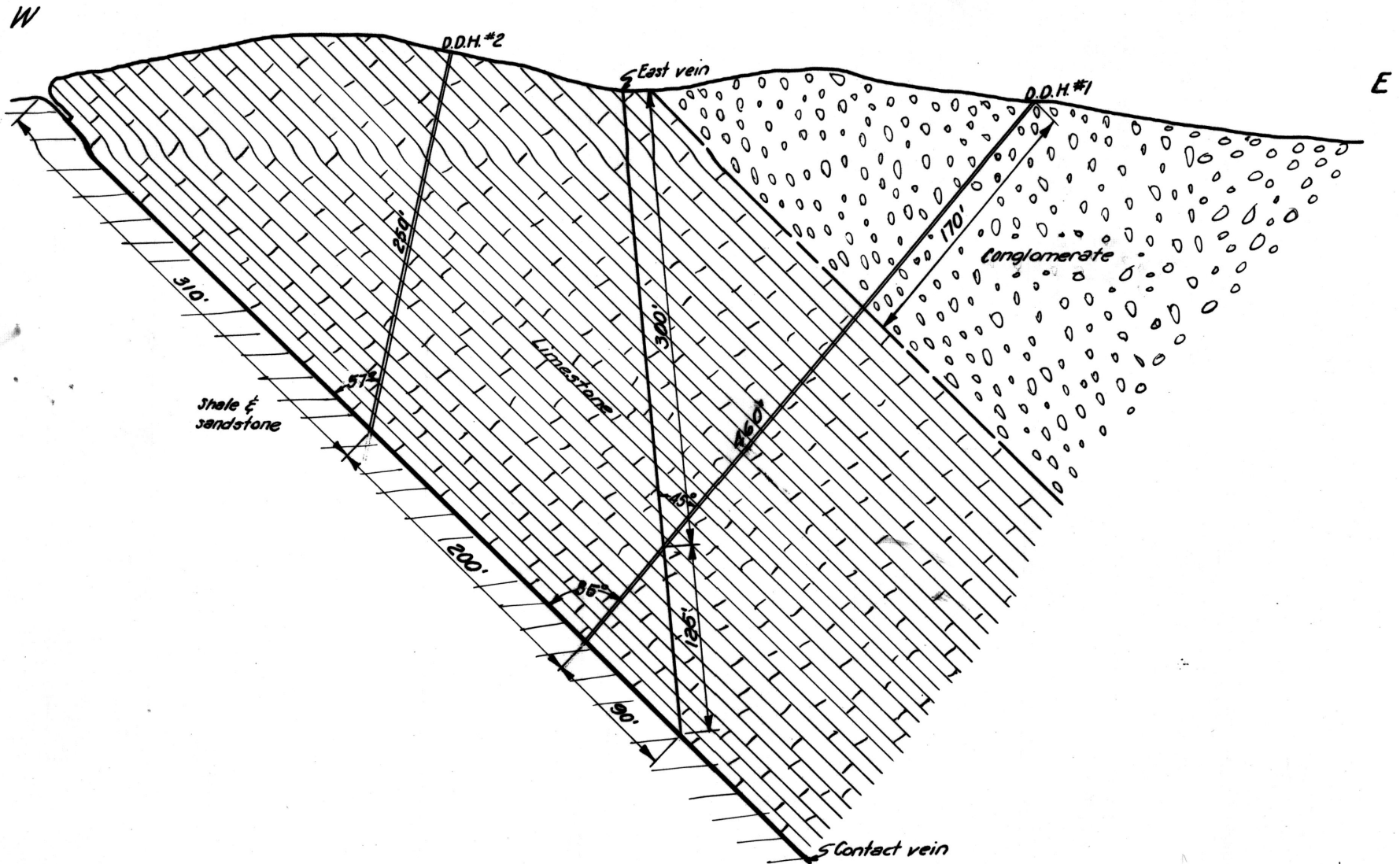
FIG. 3 - CROSS-SECTION EAST FROM STOPE AT NO. 1 SHAFT
