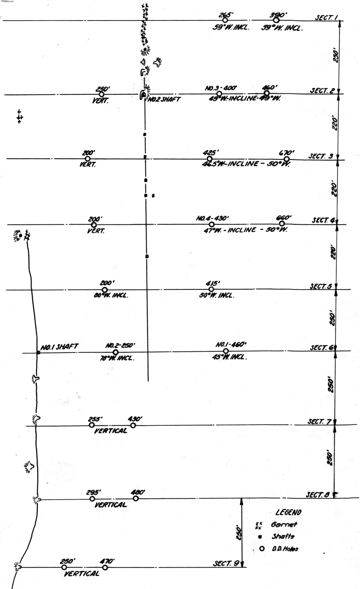
FIG. 5 - PATTERN OF PROPOSED DIAMOND DRILL HOLES
