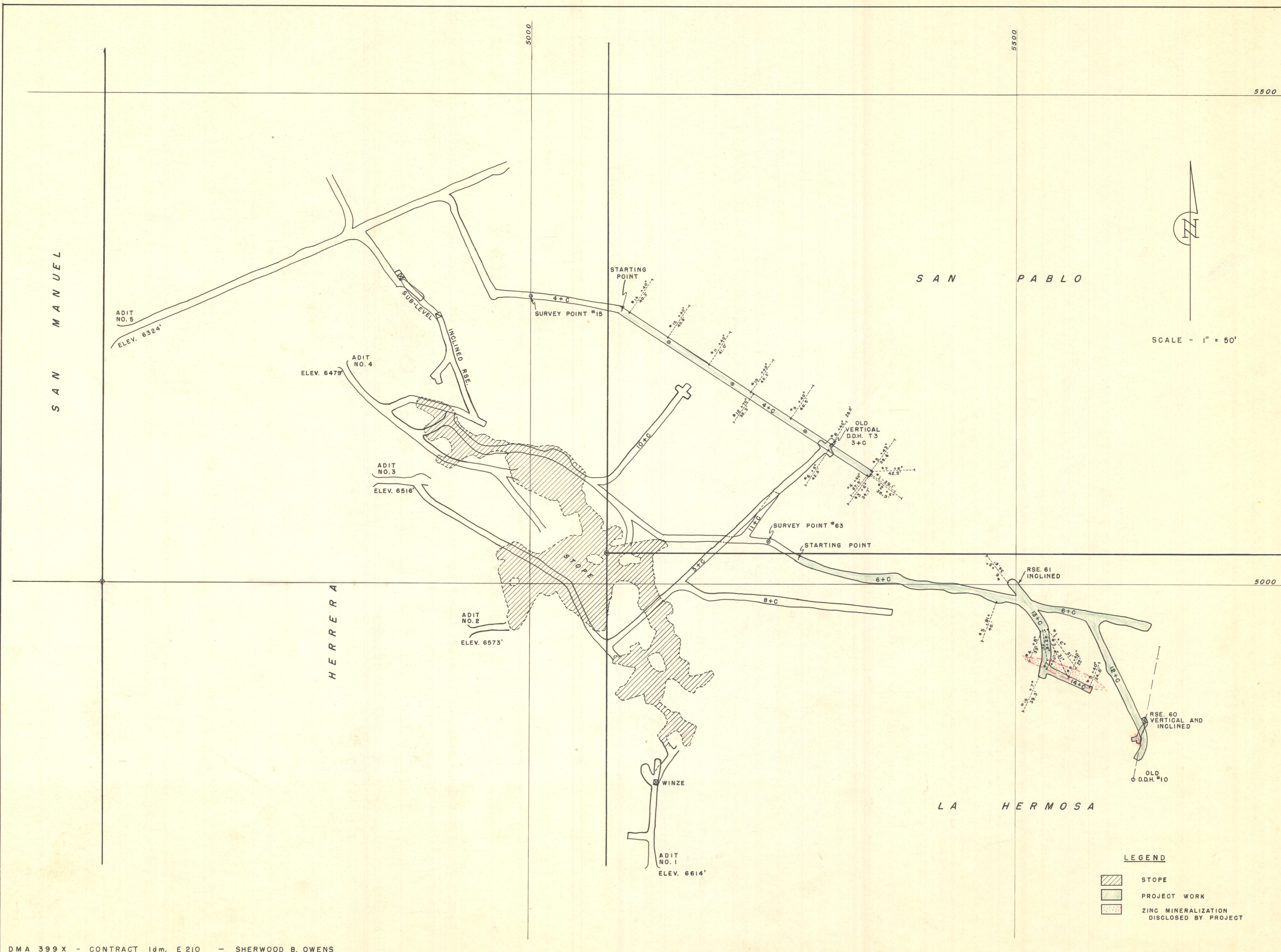
FIGURE 3. - MINE WORKINGS - ABRIL MINE - SHATTUCK-DENN MINING CORPORATION - COCHISE COUNTY, ARIZONA
