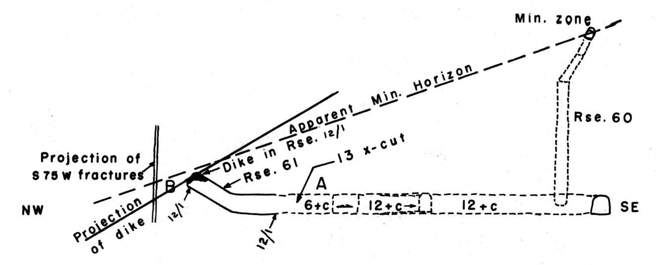
VERTICAL PROJECTION IN PLANE OF N 40 W FRACTURES
