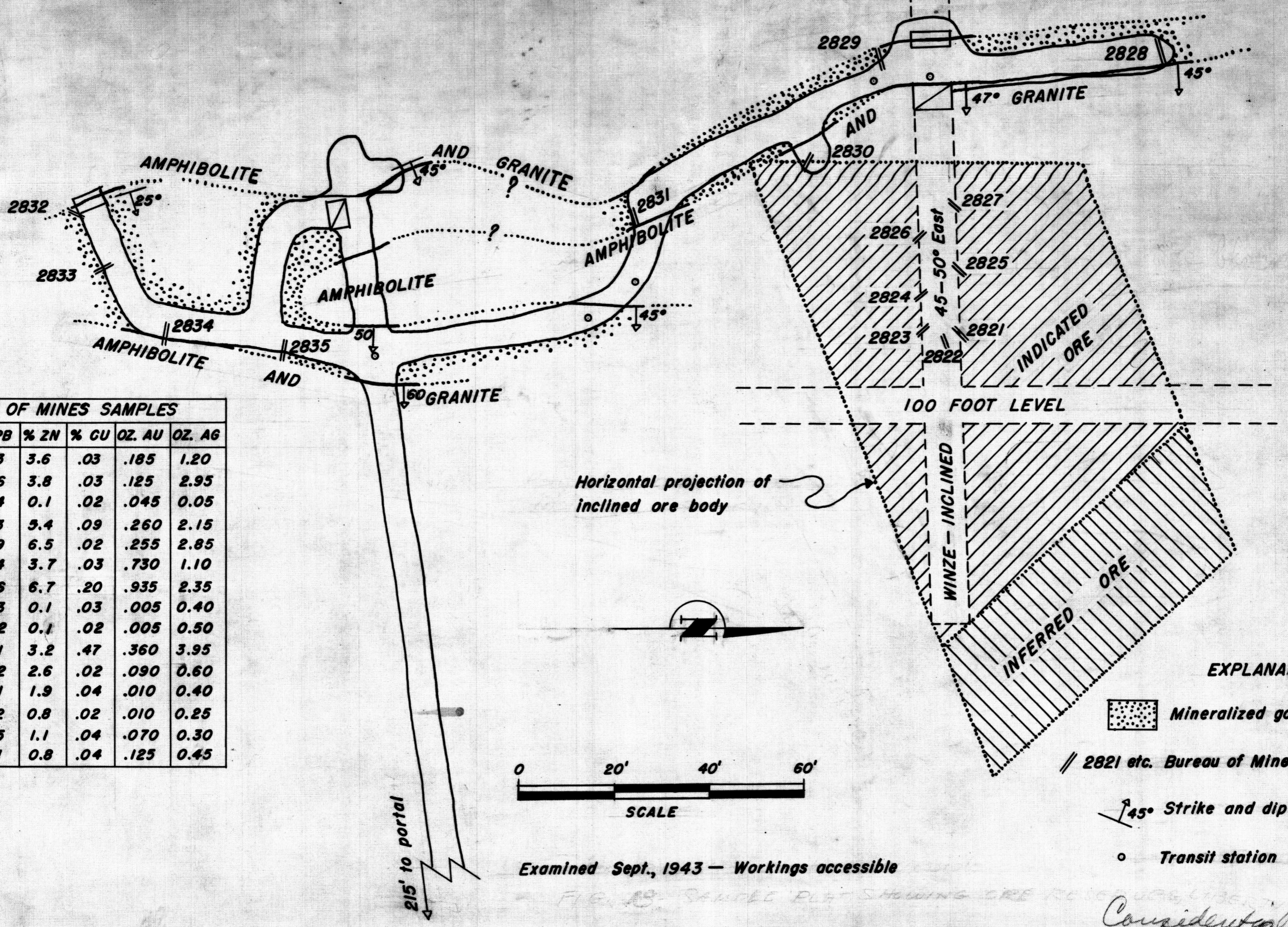
FIG. 18-SAMPLE PLAT SHOWING ORE RESERVES, LIBERTY MINE
