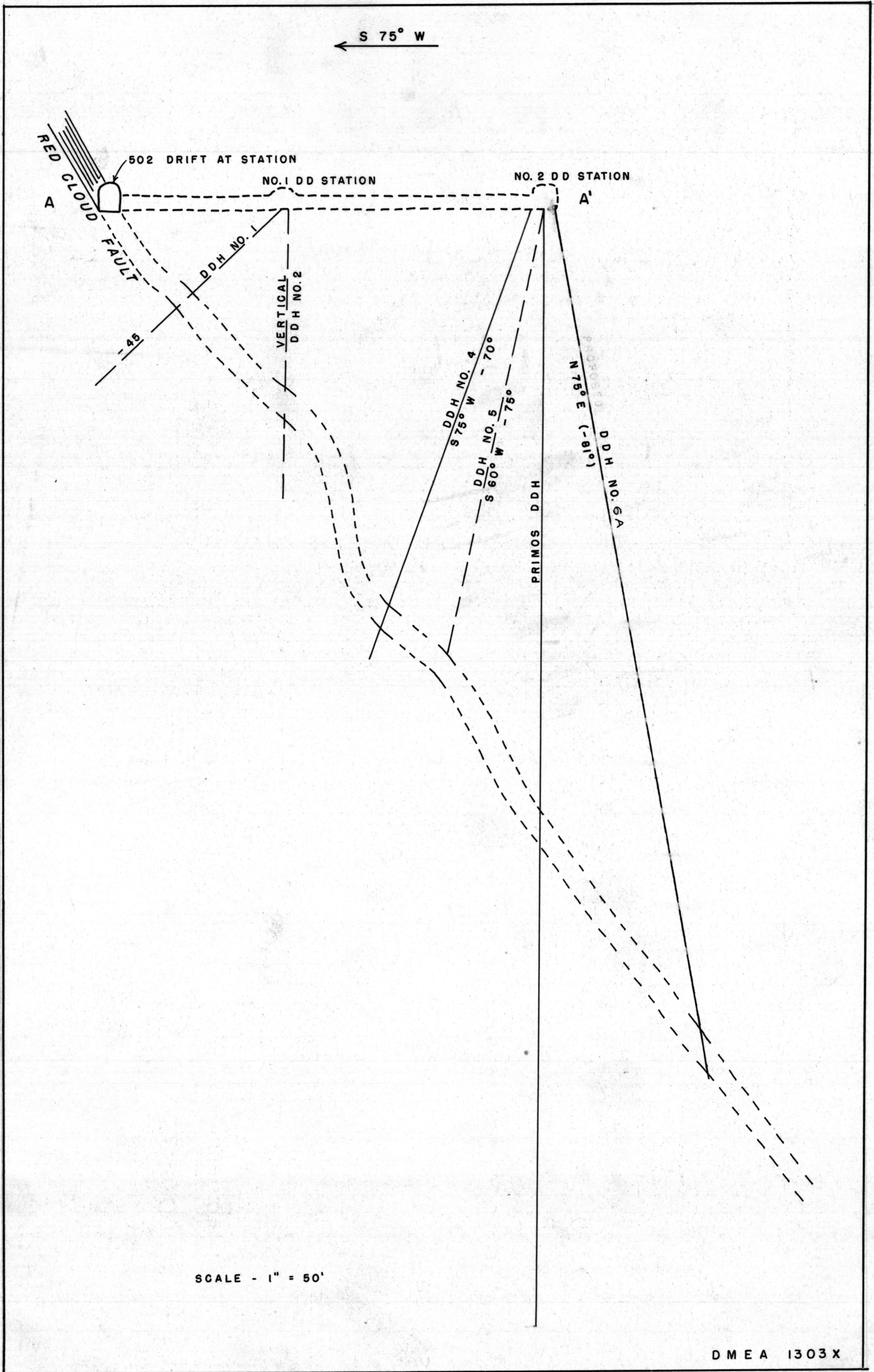
FIGURE NO. 5 SECTION ON A-A' N 75° W - RED CLOUD MINE - YUMA METALS, INC.
