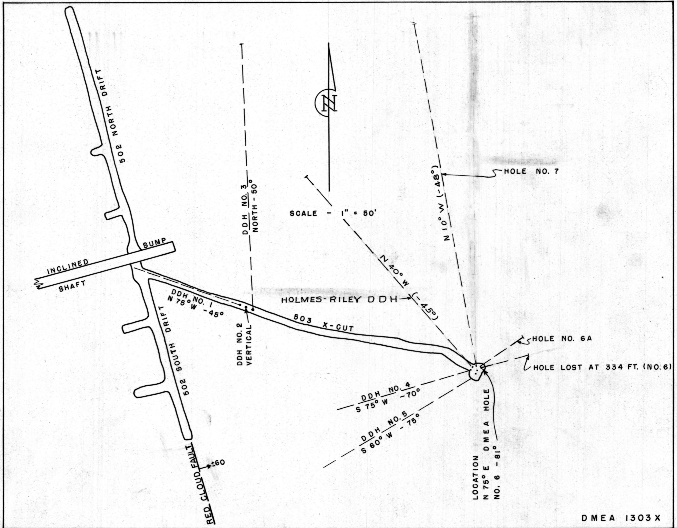
FIG. 4 500 LEVEL - RED CLOUD MINE - YUMA METALS, INC.
