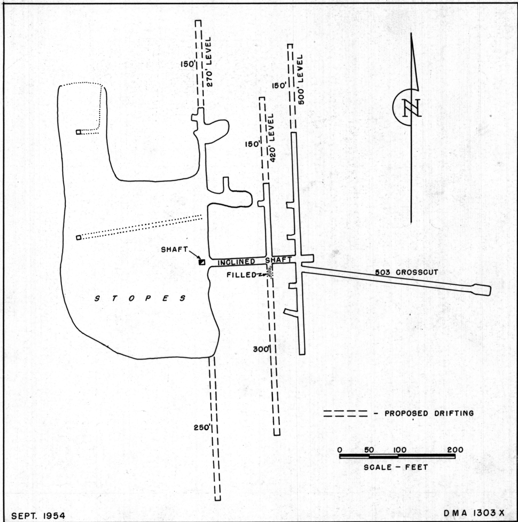
FIGURE I. - PLAN - RED CLOUD MINE - SHOWING PROPOSED DRIFTING
