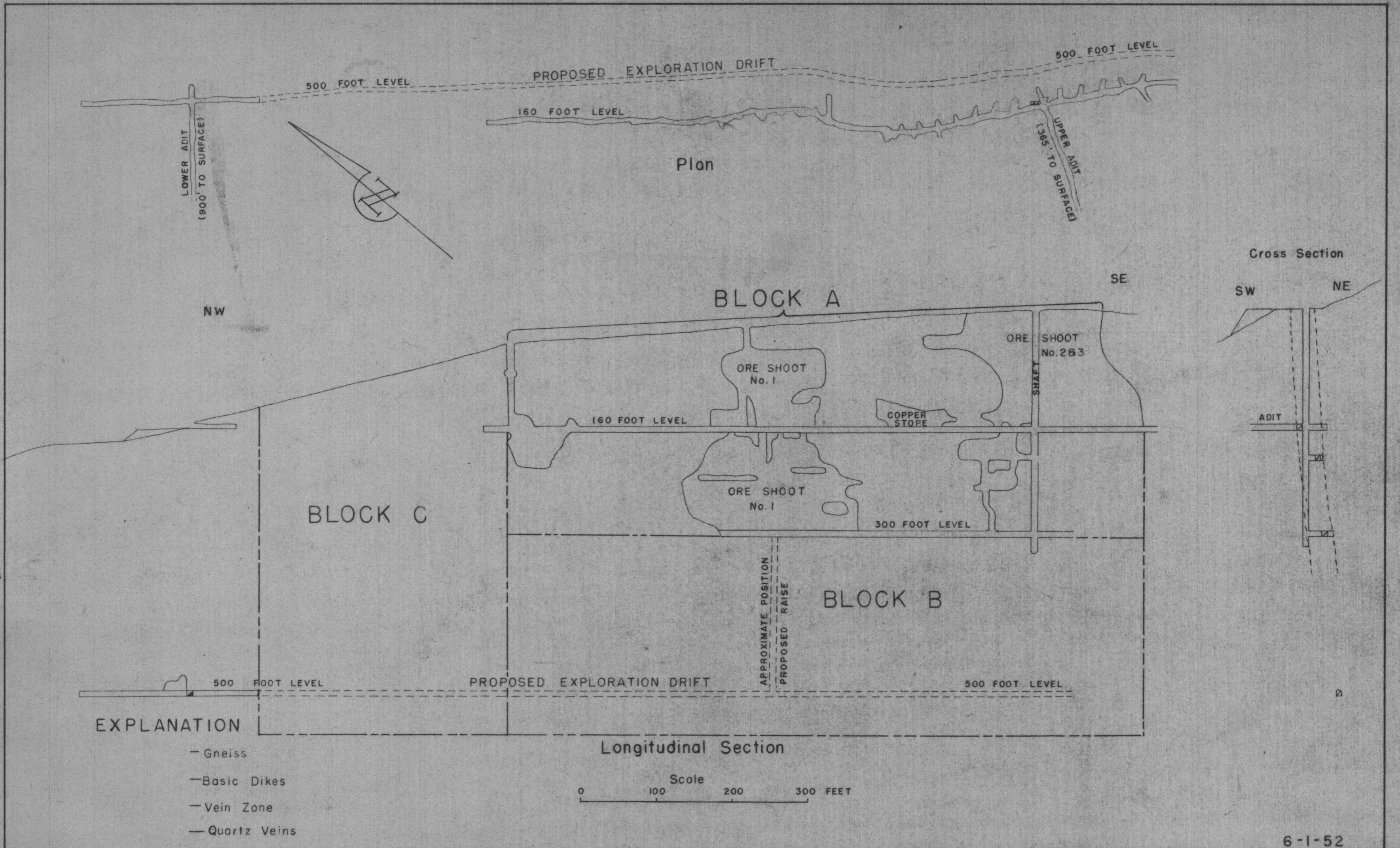
FIGURE 3-PLAN AND SECTIONS SHOWING PROPOSED EXPLORATION, SUMMIT MINE, MOHAVE COUNTY, ARIZONA
