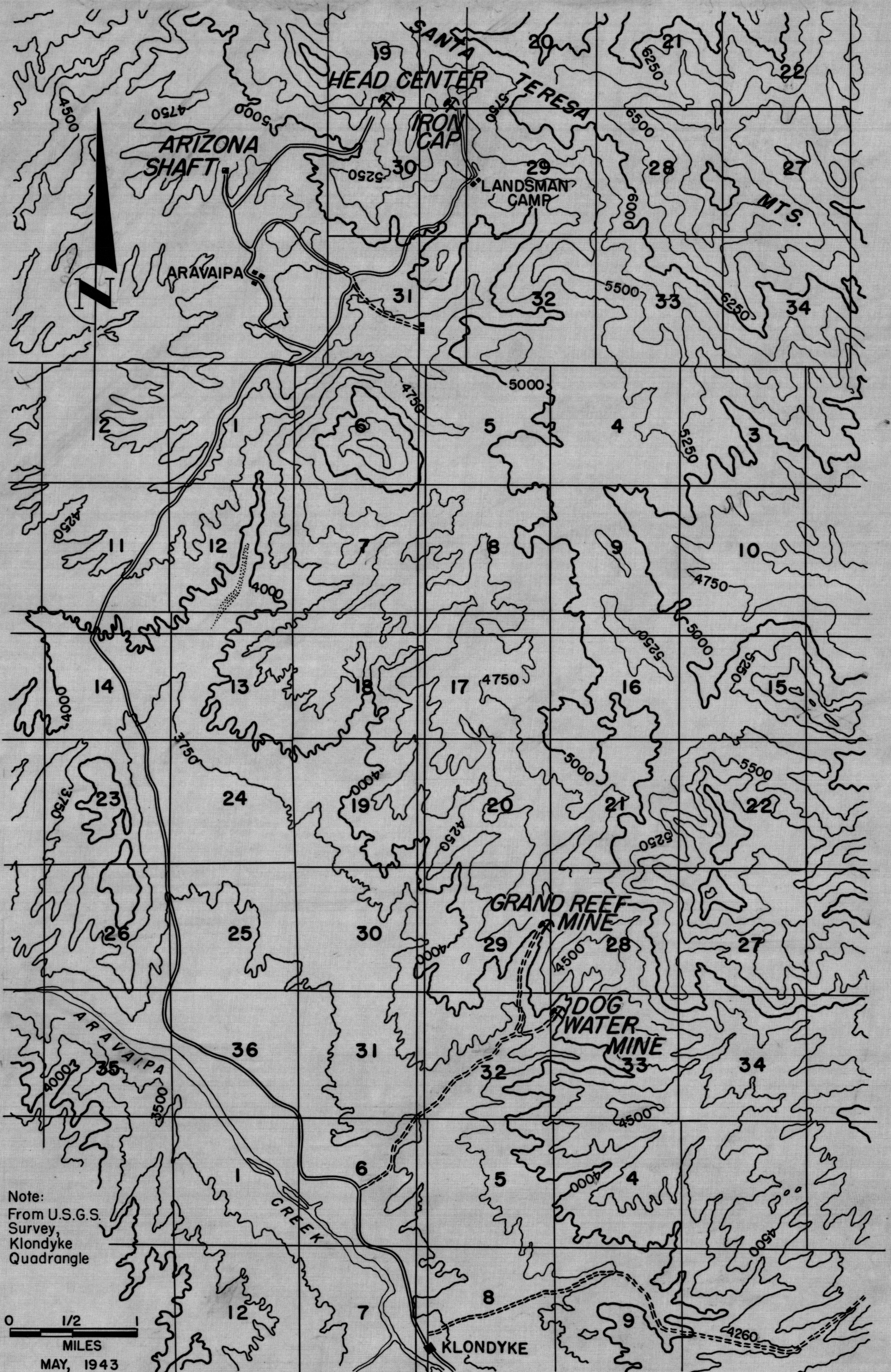
FIG.2-ARAVAIPA MINING DIST., GRAHAM CO., ARIZONA
