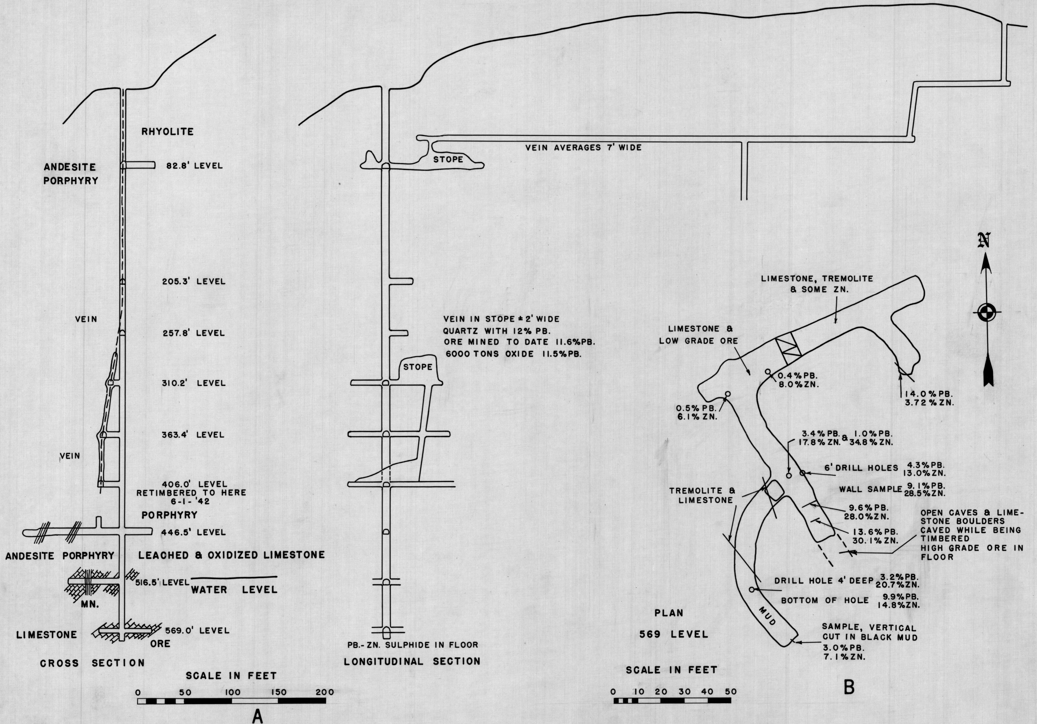
Figure 2.—Arizona mine. A, Sections through Arizona shaft; B, sample map, 569 level.
