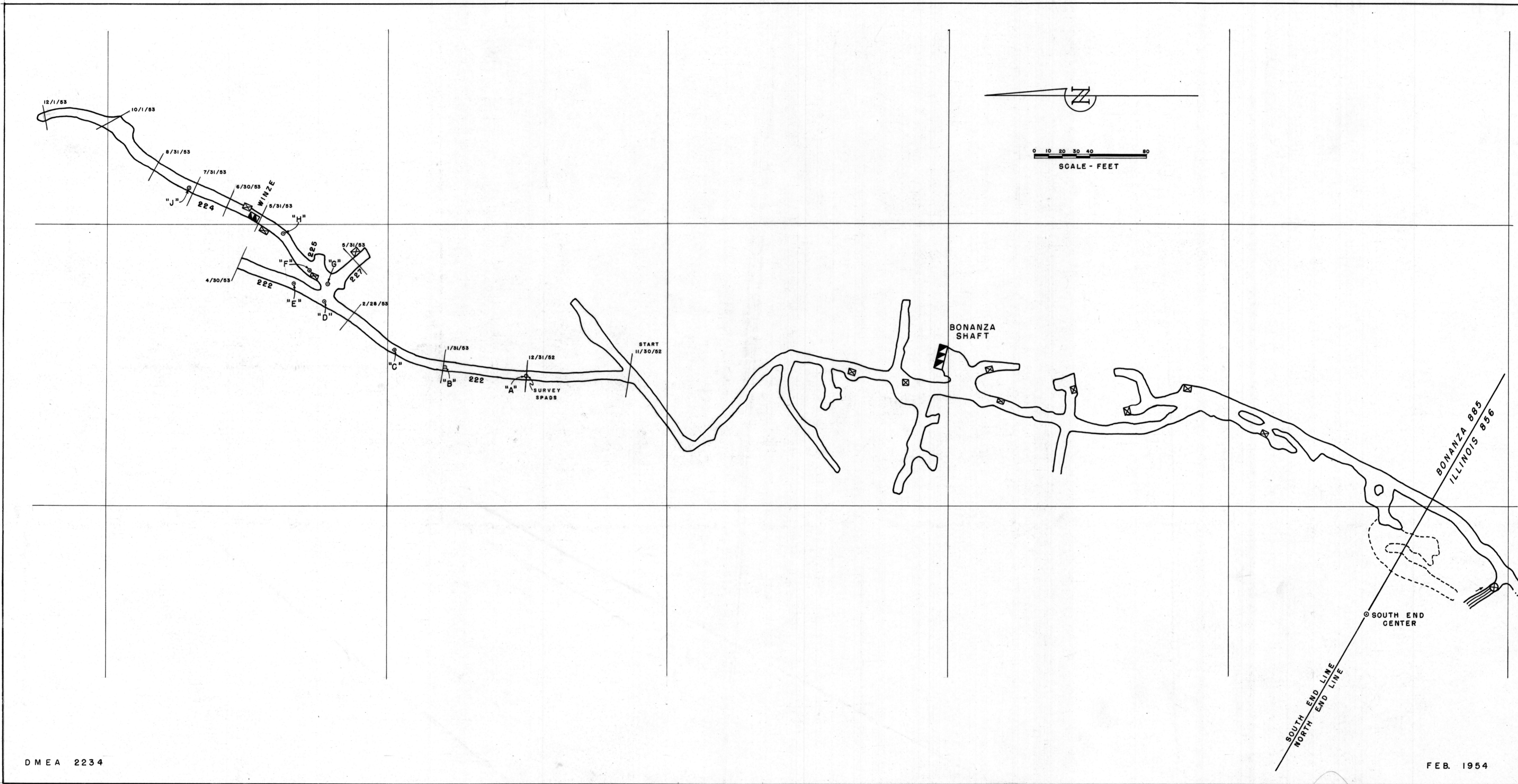
FIGURE 2. - BONANZA MINE - 235 LEVEL PATAGONIA MINING DISTRICT SANTA CRUZ COUNTY, ARIZONA
