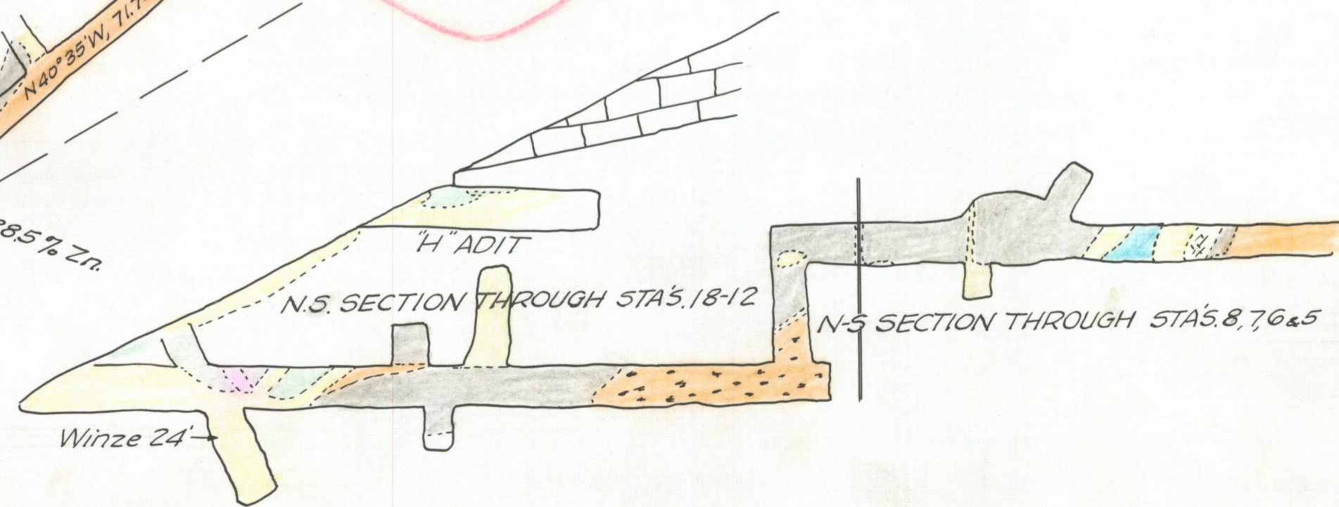
TRACED FROM MAP LOANED BY JONATHAN GORDON PLAN OF WORKINGS SIDE SHOW & VALENTINE CLAIMS SAN JUAN GROUP COCHISE COUNTY, ARIZ. SCALE: 1" = 30' S.W. Voelzel ENGINEER FIG. 4
