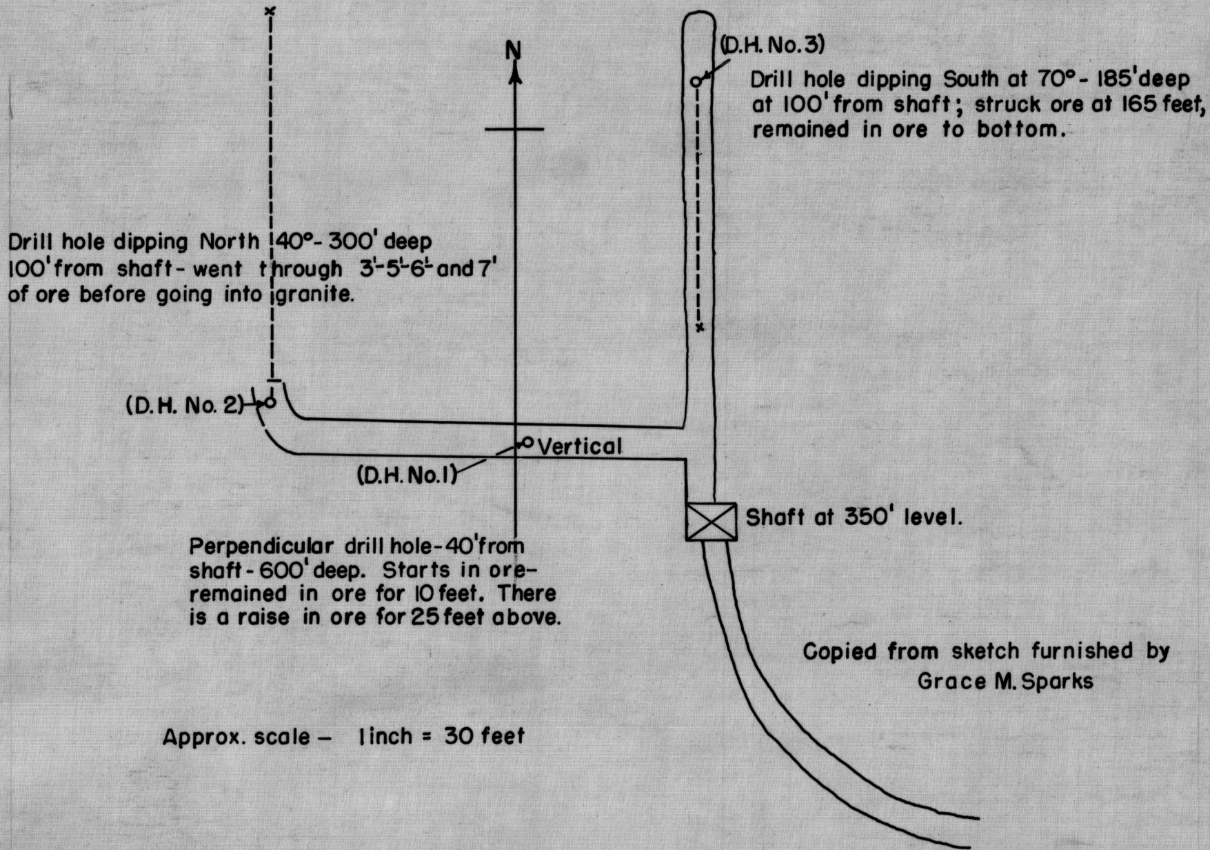
Fig. 6.— Plan of the work in the bottom of the shaft — State of Texas Property.
