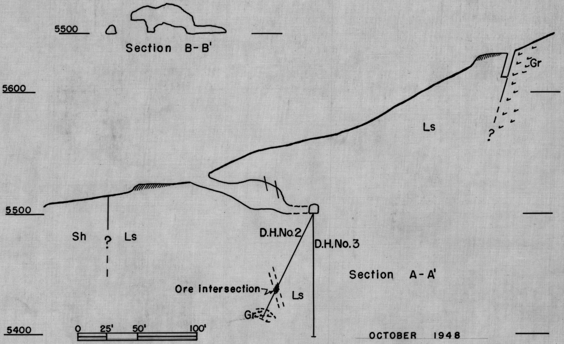
Figure 5.- Sections - State of Texas mine.
