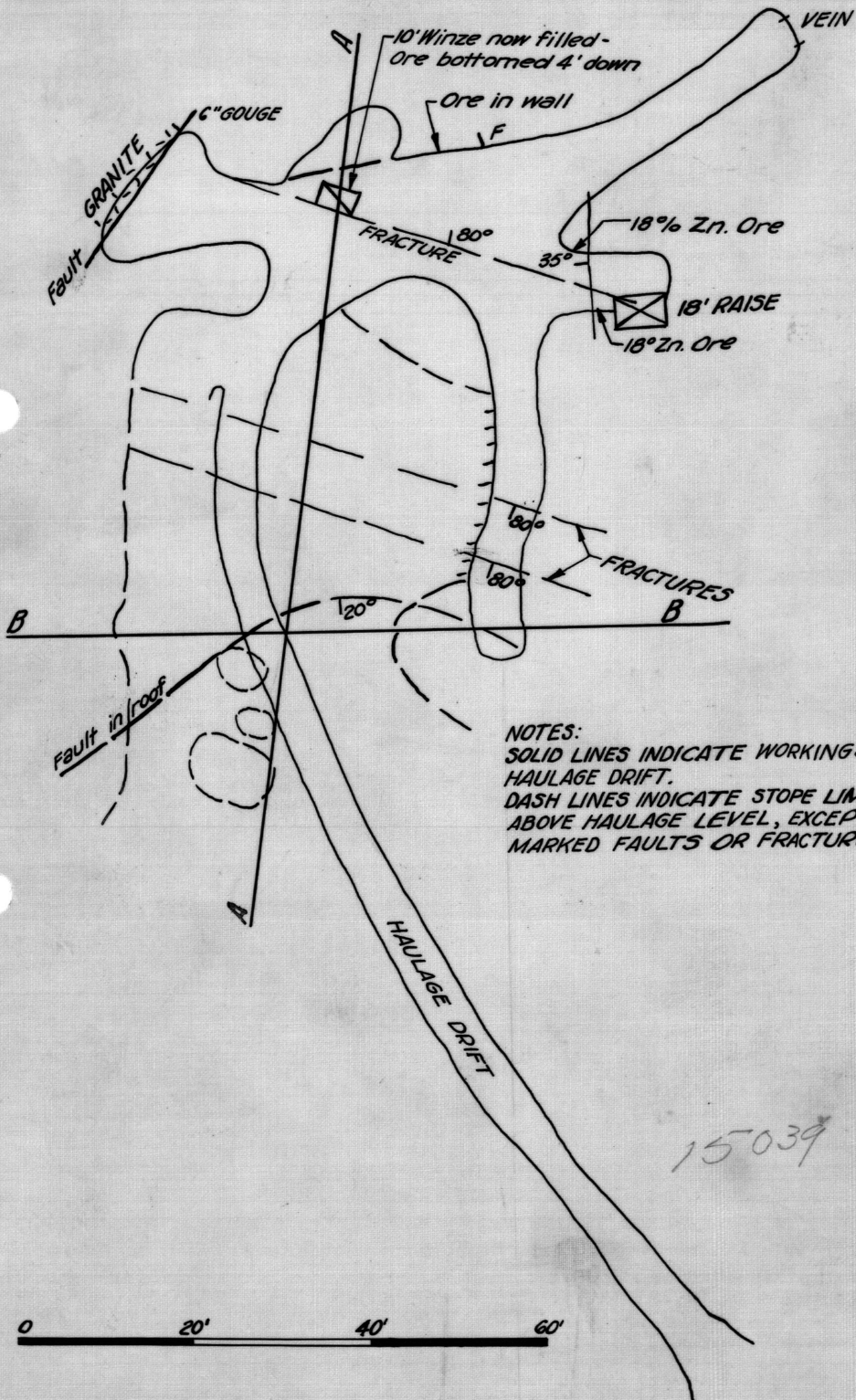
FIG.2-UNDERGROUND WORKINGS-STATE OF TEXAS MINE
