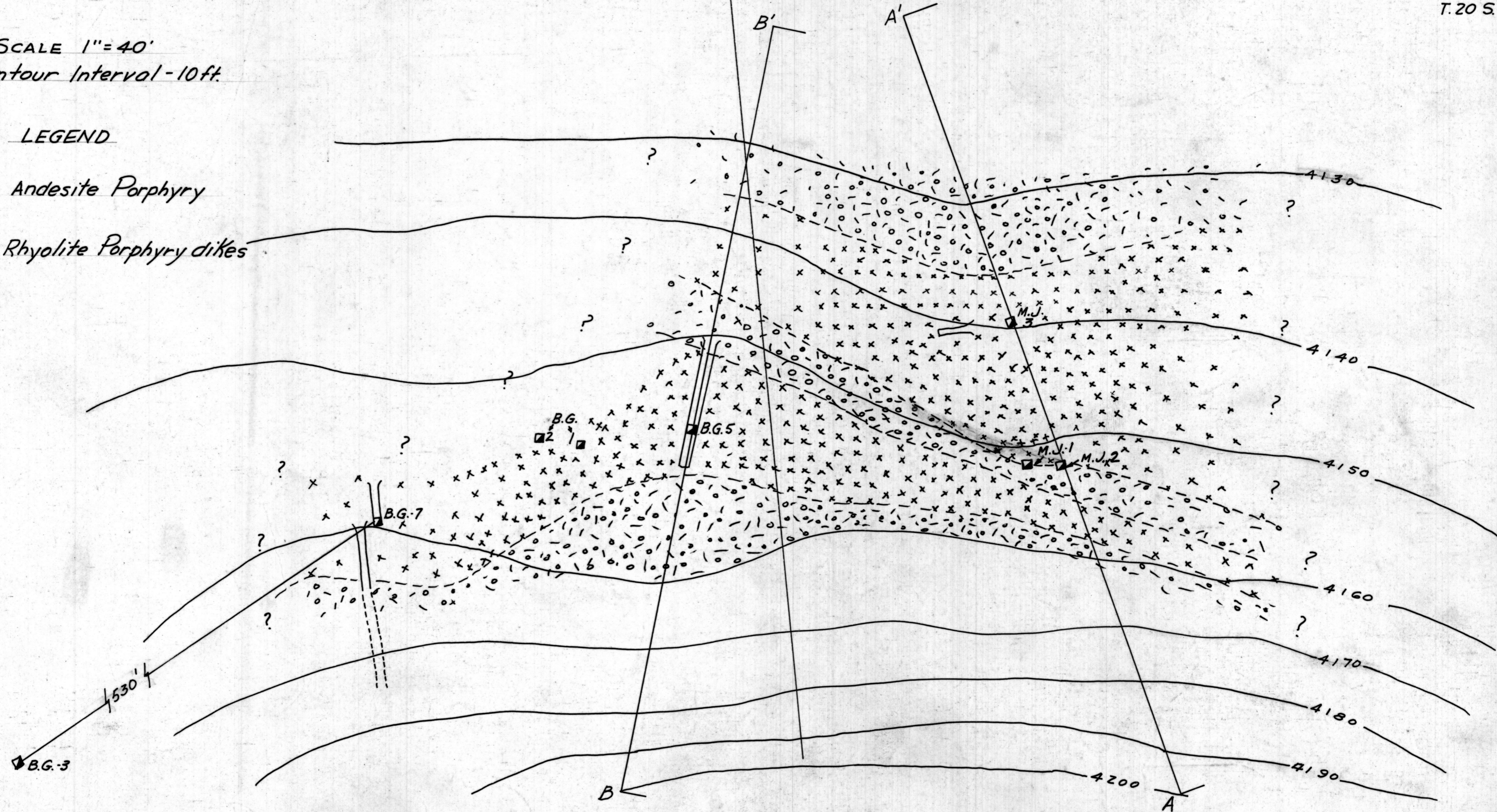
Figure 3.- Sketch of topography and geology, Brother George and Mary Jo claims, Grant mine, Cochise County, Arizona.
