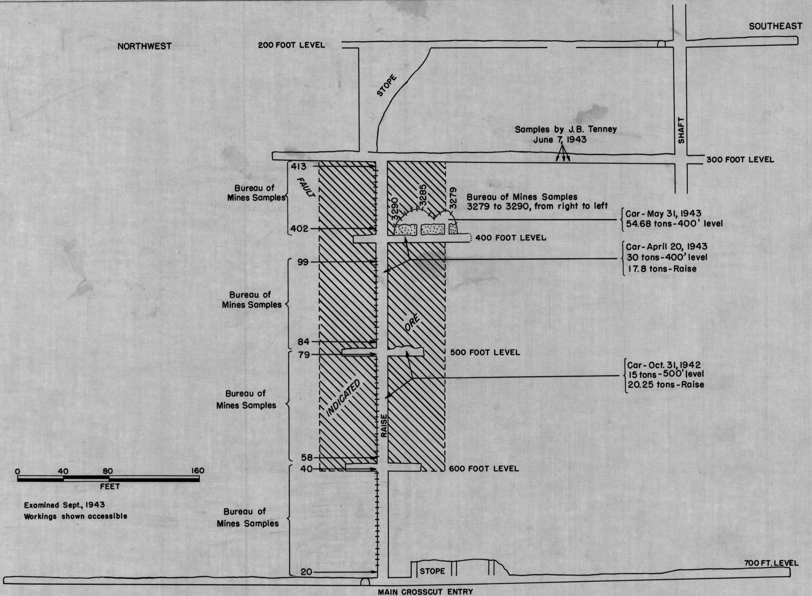
FIG. 20-SAMPLE PLAT SHOWING ORE RESERVES, BRIGHTER DAYS MINE
