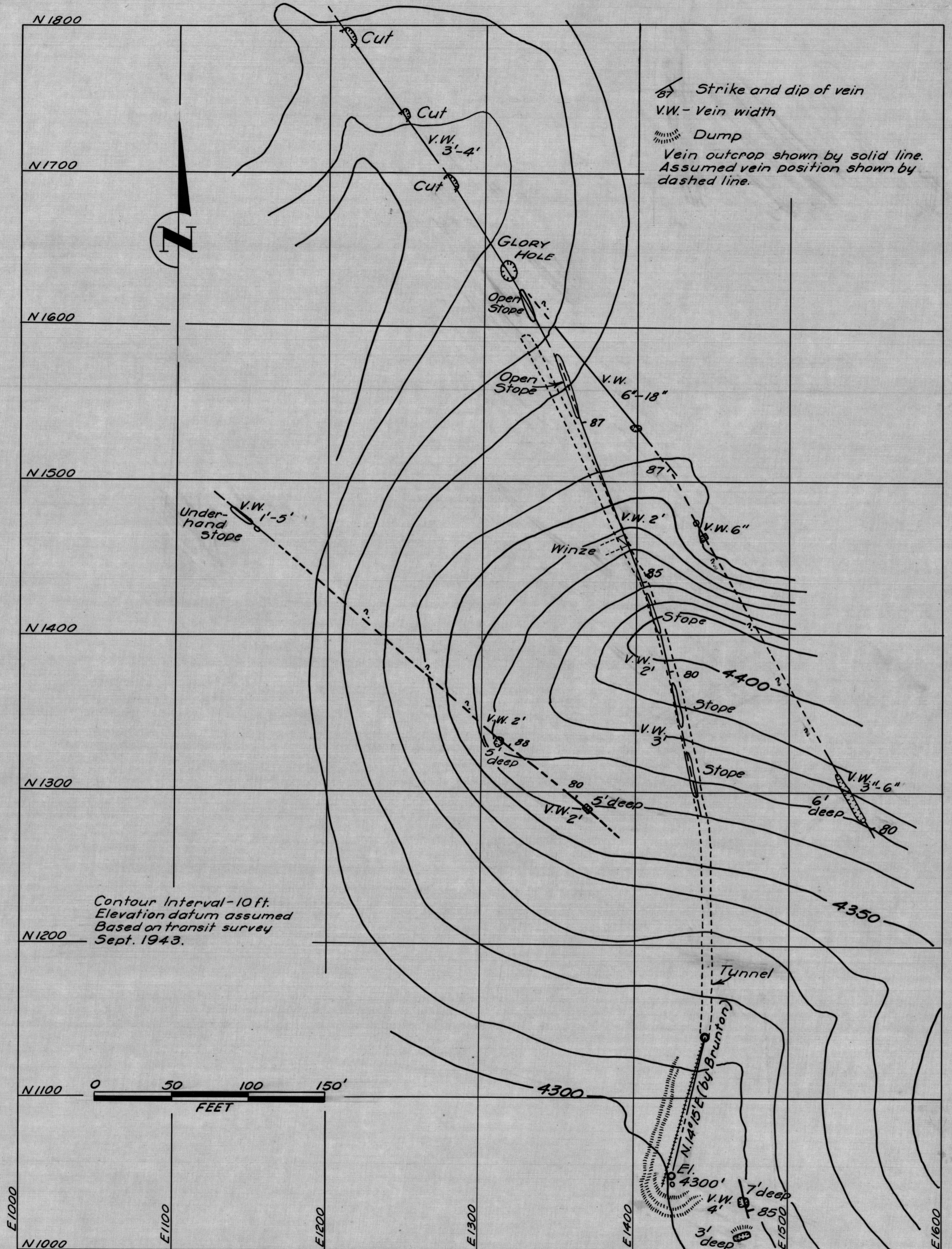
FIG. 14 - TOPOGRAPHIC MAP OF COLUMBUS LEAD ZINC MINE, MOHAVE CO., ARIZONA
